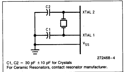
Figure 3. Oscillator Connections
