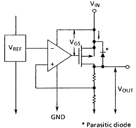
Figure 13 Control transistor
