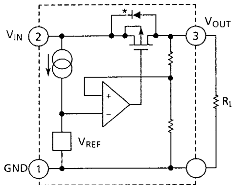
Figure 2 * Parasitic diode
