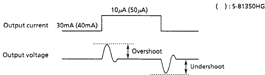
Figure 12 Ringing waveform
