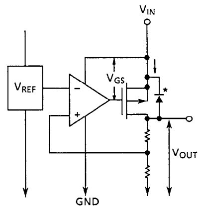
Figure 7 Control transistor
