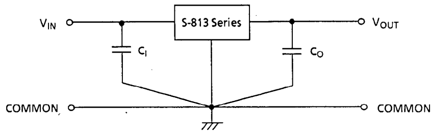
Figure 20 Standard circuit
