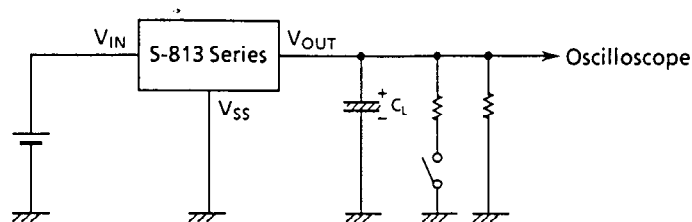
Figure 13 Measuring circuit
