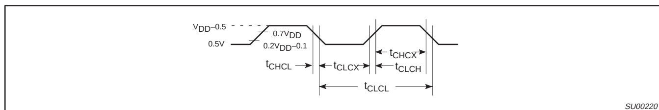
Figure 13. Clock Signal Waveform for I_{DD} Tests in Active and Idle Modes t_{CLCH} = t_{CHCL} = 5\text{ns}
