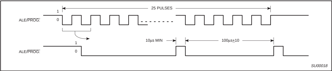
Figure 16. PROG Waveform
