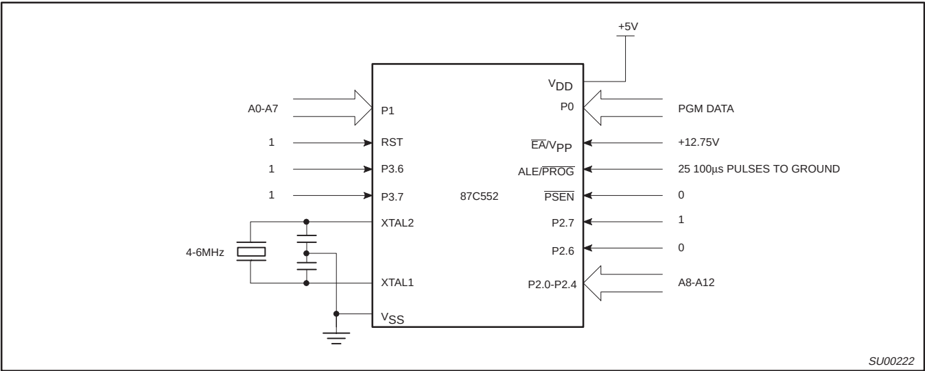
Figure 15. Programming Configuration
