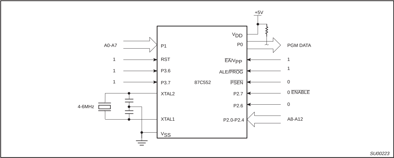
Figure 17. Program Verification
