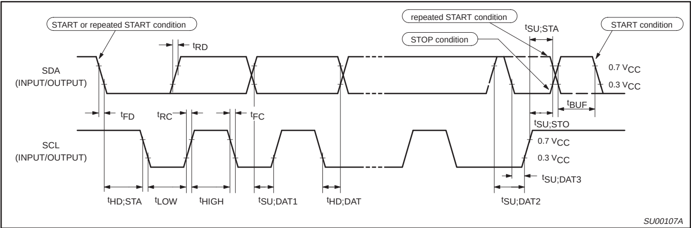
Figure 9. Timing SIO1 (I²C) Interface
