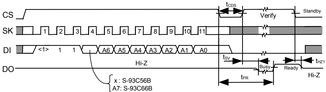
Figure 13 Data Erase Timing (S-93C56B, S-93C66B)
