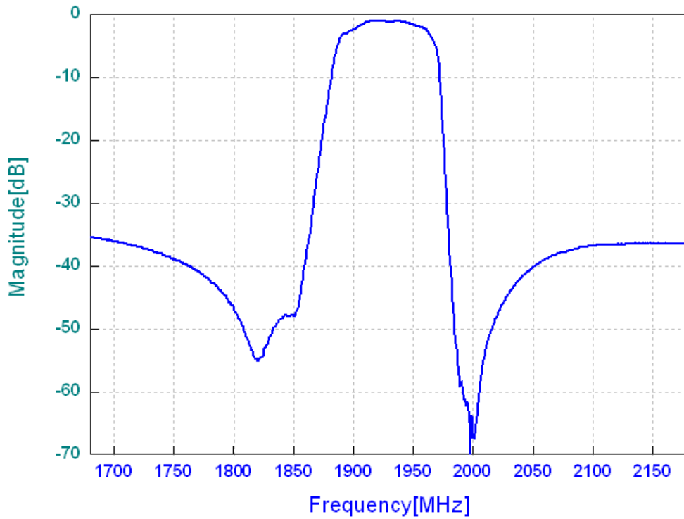
Frequency Response
