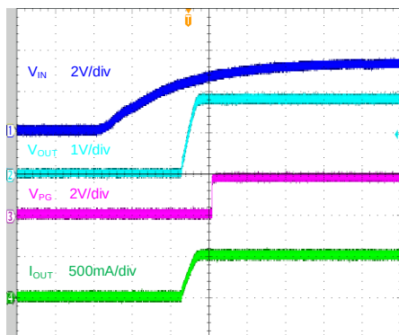
Startup from V_{IN} ( V_{IN}=V_{EN}=3.3V , V_{OUT}=1.8V , I_{OUT}=0.5A , C_{IN}=1\mu F , C_{OUT}=2.2\mu F )
