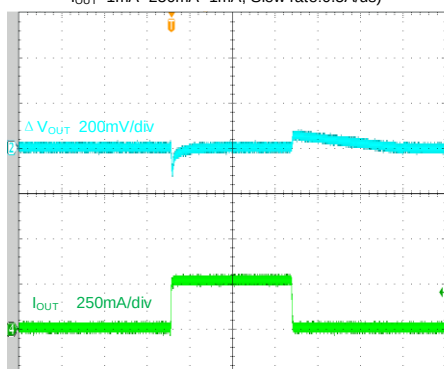
Load Transient ( V_{IN}=3.3V , V_{OUT}=1.8V , C_{IN}=1\mu F , C_{OUT}=2.2\mu F , C_{FF}=100pF , I_{OUT}=1mA \sim 250mA \sim 1mA , Slew rate: 0.5A/us)
