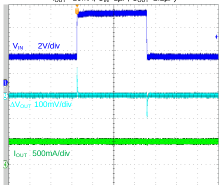
Line Transient ( V_{IN}=2.3V \sim 6V \sim 2.3V , Slew rate: 1V/us, V_{OUT}=1.8V , I_{OUT}=10mA , C_{IN}=1\mu F , C_{OUT}=2.2\mu F )
