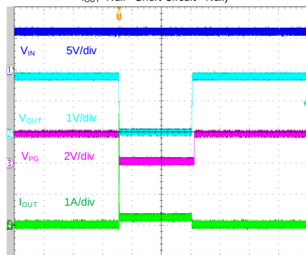
Short Circuit Protection ( V_{IN}=6V , V_{OUT}=1.8V , C_{IN}=1\mu F , C_{OUT}=2.2\mu F , I_{OUT}=Null \sim Short\ Circuit \sim Null )
