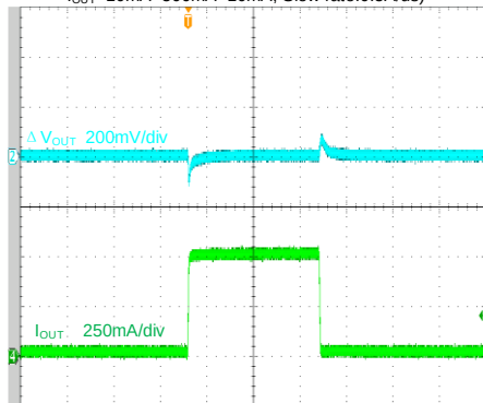
Load Transient ( V_{IN}=3.3V , V_{OUT}=1.8V , C_{IN}=1\mu F , C_{OUT}=2.2\mu F , C_{FF}=100pF , I_{OUT}=10mA \sim 500mA \sim 10mA , Slew rate: 0.5A/us)
