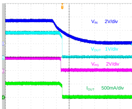
Shutdown from V_{IN} ( V_{IN}=V_{EN}=3.3V , V_{OUT}=1.8V , I_{OUT}=0.5A , C_{IN}=1\mu F , C_{OUT}=2.2\mu F )
