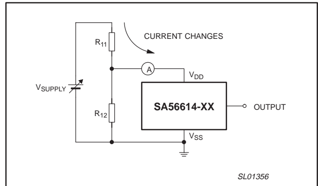
Figure 15. High impedance supply operating problems
