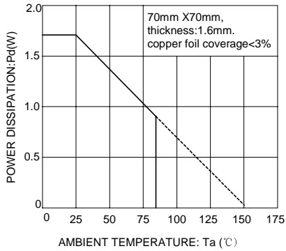
Fig 1. Thermal dissipation curve
