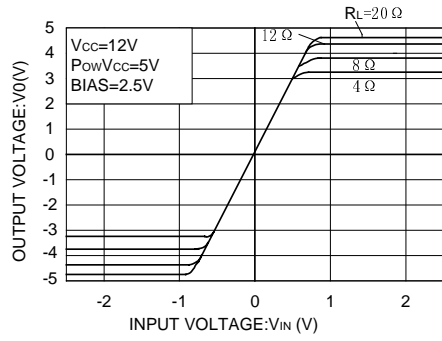
Fig 4. Driver I/O characteristics (slew)
