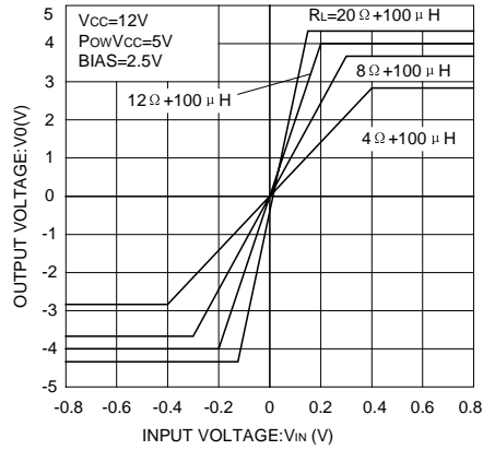
Fig 2. Driver I/O characteristics (focus and tracking)
