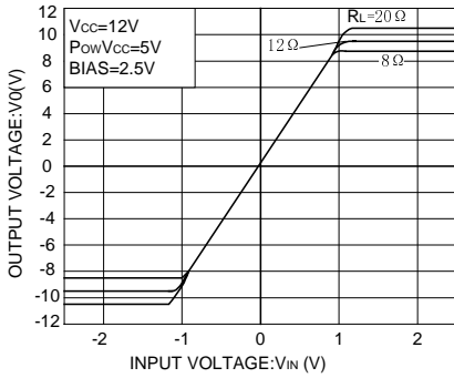
Fig 3. Driver I/O characteristics (Loading)
