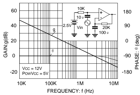
Fig 6. Op-amp phase-frequency, amplitude-frequency characteristics
