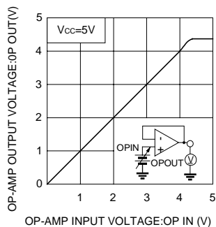
Fig 5. Op-amp I/O characteristics
