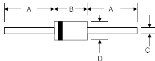
DO-15
