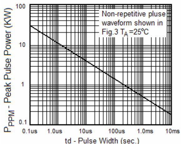
Fig5. Peak Pulse Power Rating curve
