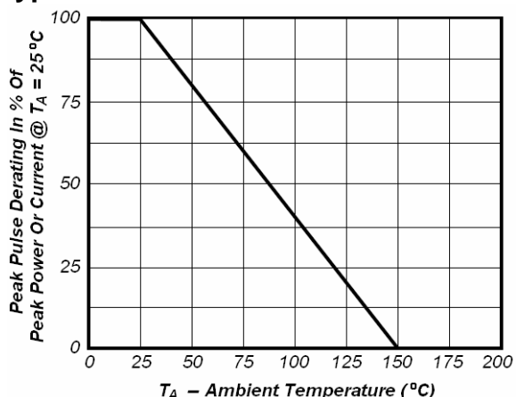
Fig1. Pulse Dearing Curve
