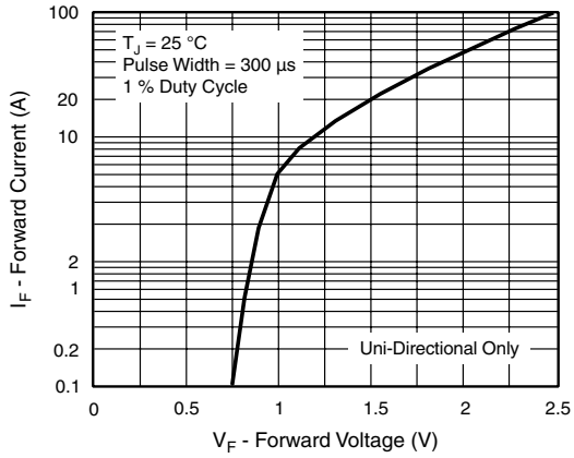
Figure 11. Typical Instantaneous Forward Voltage
