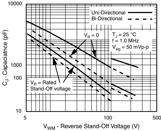
Figure 6. Capacitance
