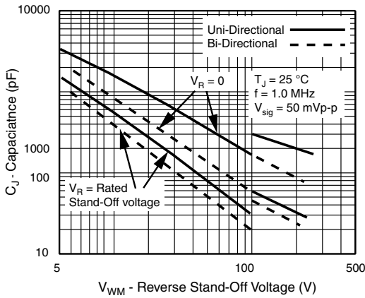
Figure 6. Capacitance
