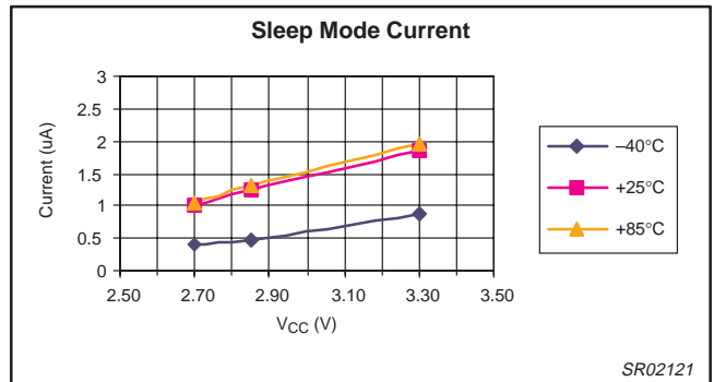
Figure 8. Sleep Mode Current
