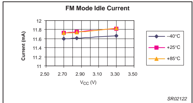
Figure 7. FM Mode Idle Current
