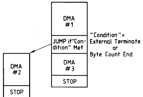
c) Conditional DMA Operation
