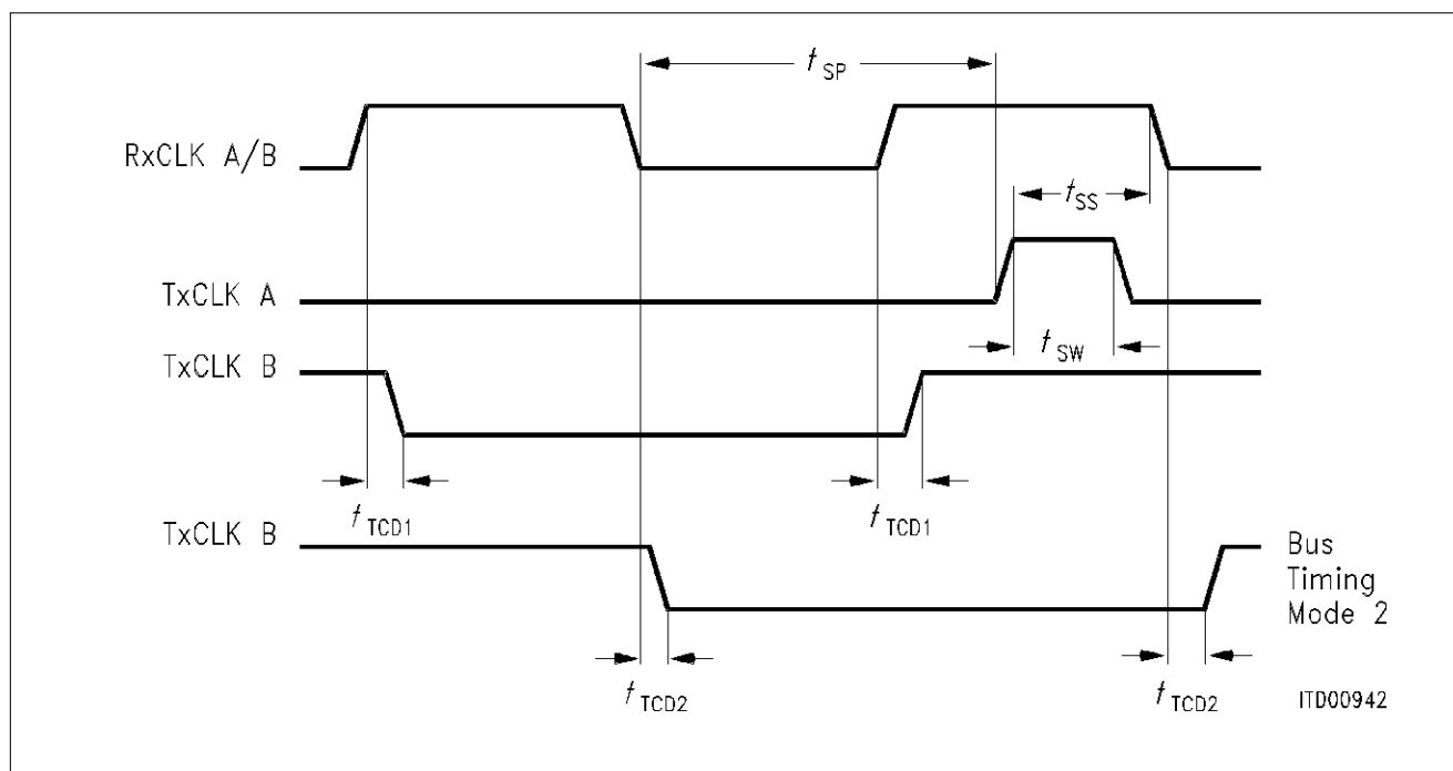
Figure 29 Clock Mode 5
