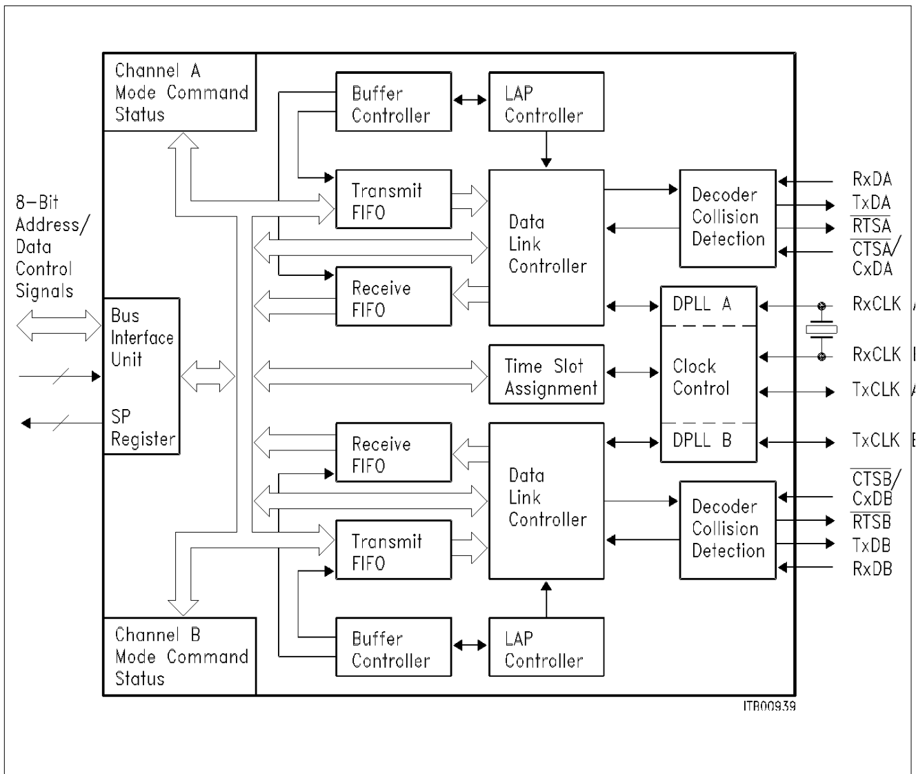
Figure 4 Block Diagram
