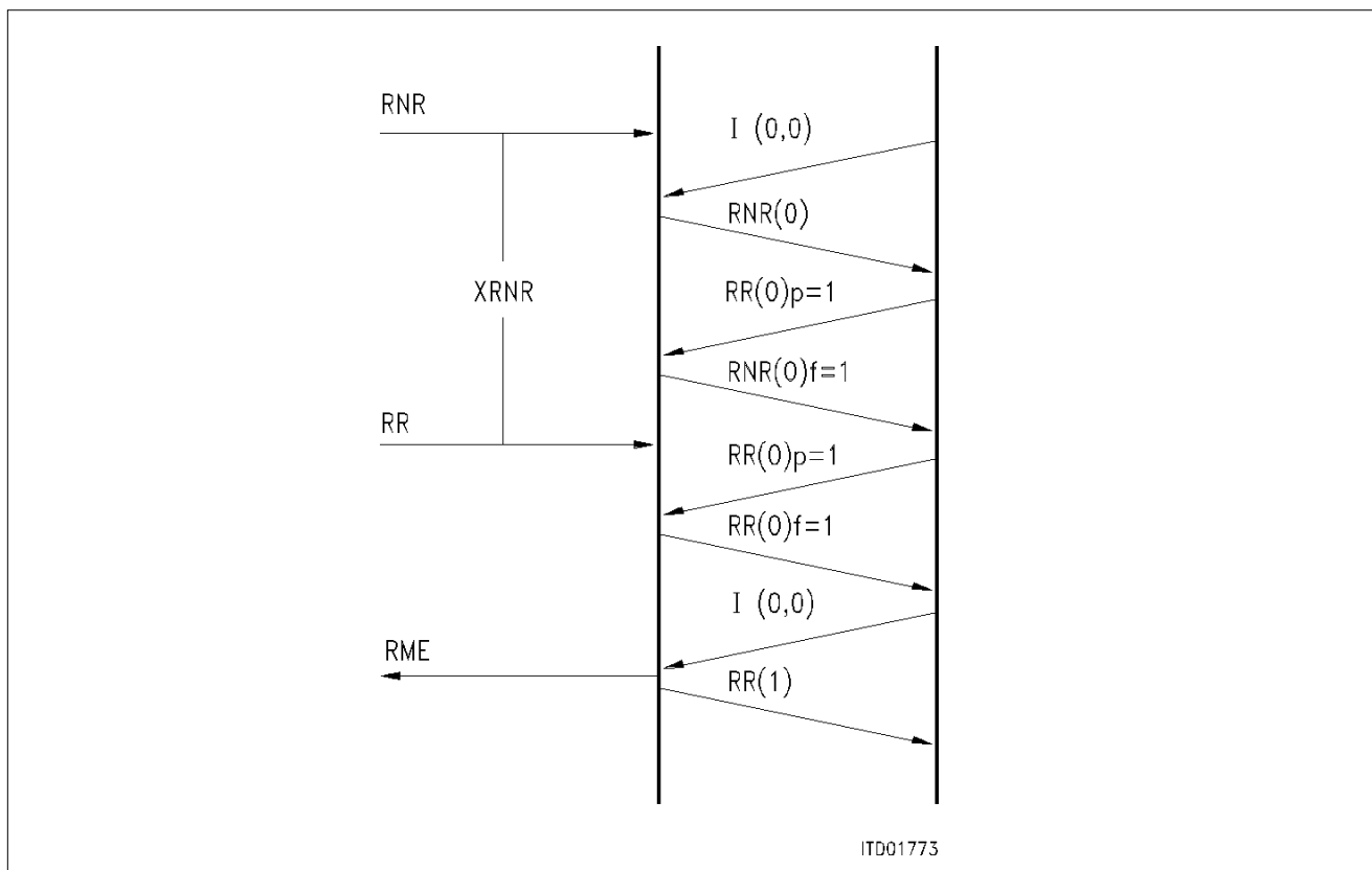
Figure 19 Flow Control with RR/RNR: Receiving I Frame
