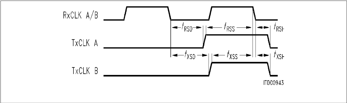
Figure 30 Clock Mode 1
