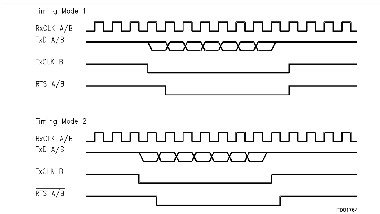
Figure 11 Transmission of 56 Kbit Channels Bus Mode
