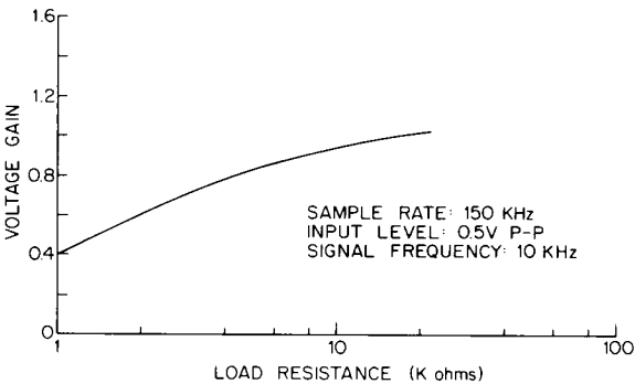
Figure 7. Dependence of Gain on Load Resistance.
