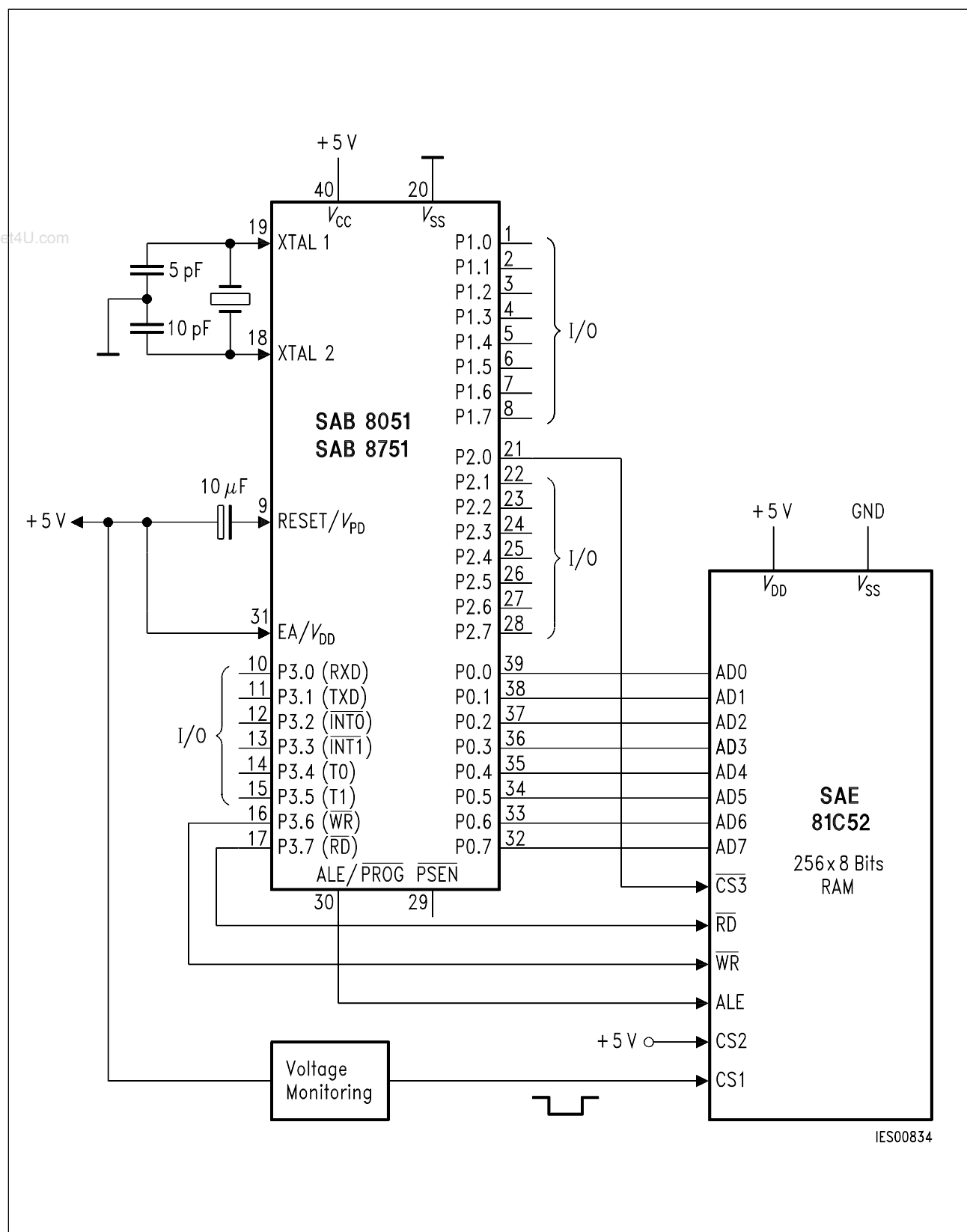
Application Circuit SAE 81C52 with the \mu C SAB 8051
