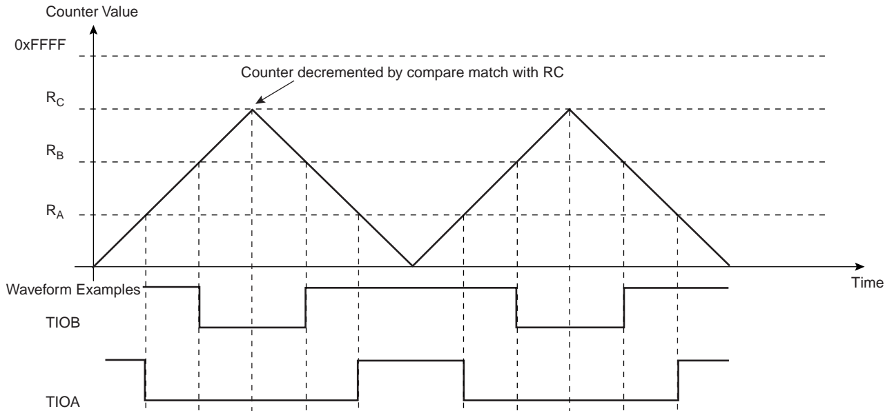
Figure 38-13. WAVSEL = 11 Without Trigger
