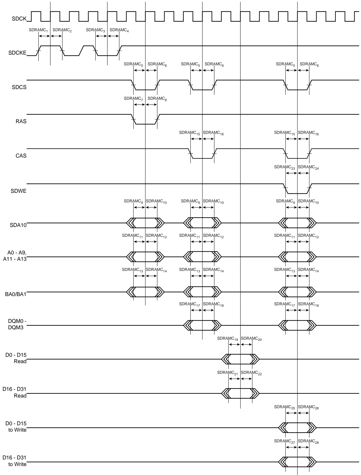
Figure 46-6. SDRAMC Signals Relative to SDCK
