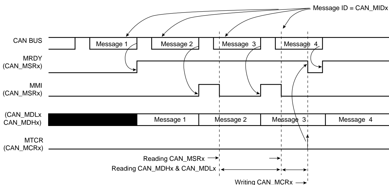
Figure 36-12. Receive with Overwrite Mailbox
