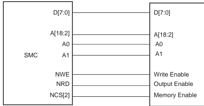
Figure 21-4. Memory Connection for a 16-bit Data Bus
