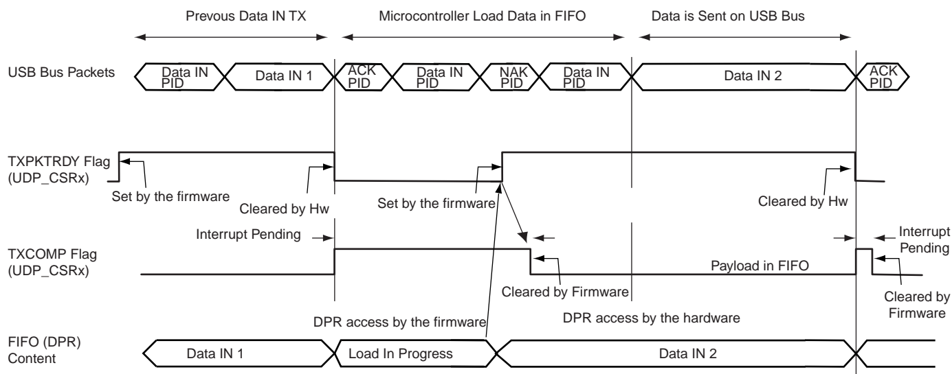
Figure 42-6. Data IN Transfer for Non Ping-pong Endpoint
