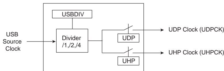
Figure 27-2. USB Clock Controller
