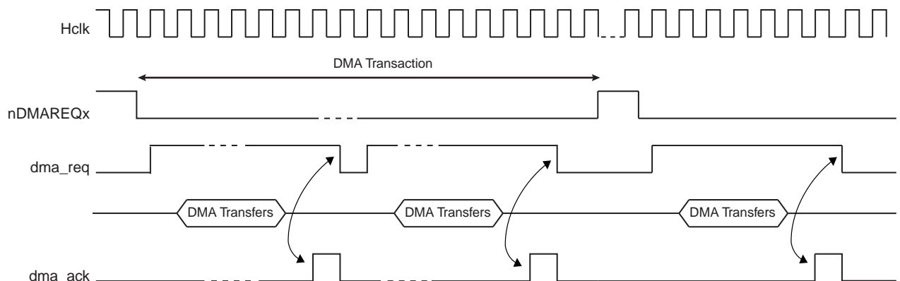
Figure 24-4. External DMA Request Timing
