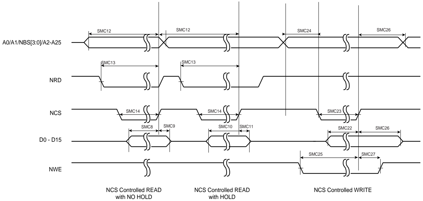
Figure 46-4. SMC timings - NCS controlled Read and Write
