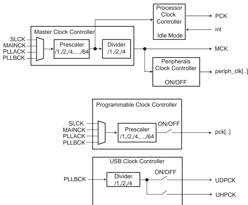
Figure 8-3. SAM9263 Power Management Controller Block Diagram
