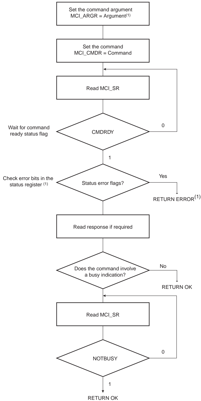
Figure 39-9. Command/Response Functional Flow Diagram
