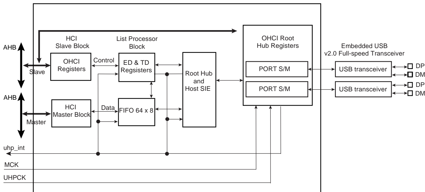
Figure 41-1. Block Diagram
