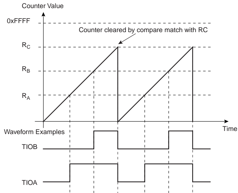
Figure 38-9. WAVSEL = 10 Without Trigger
