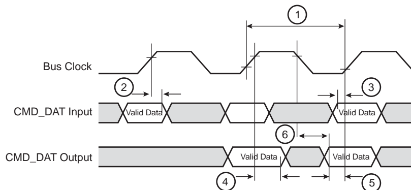
Figure 46-15. MCI Timing Diagram
