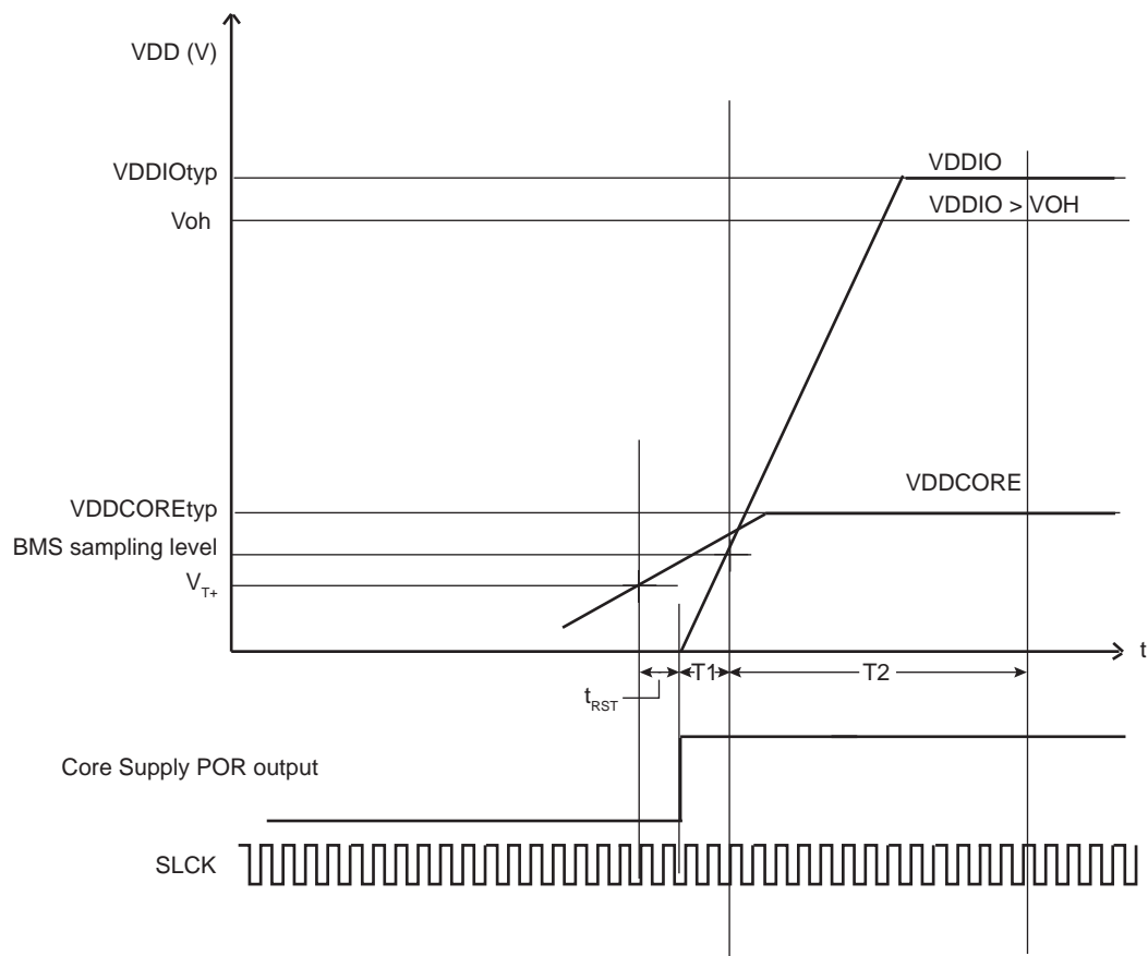
Figure 4-1. VDDCORE and VDDIO Constraints at Startup
