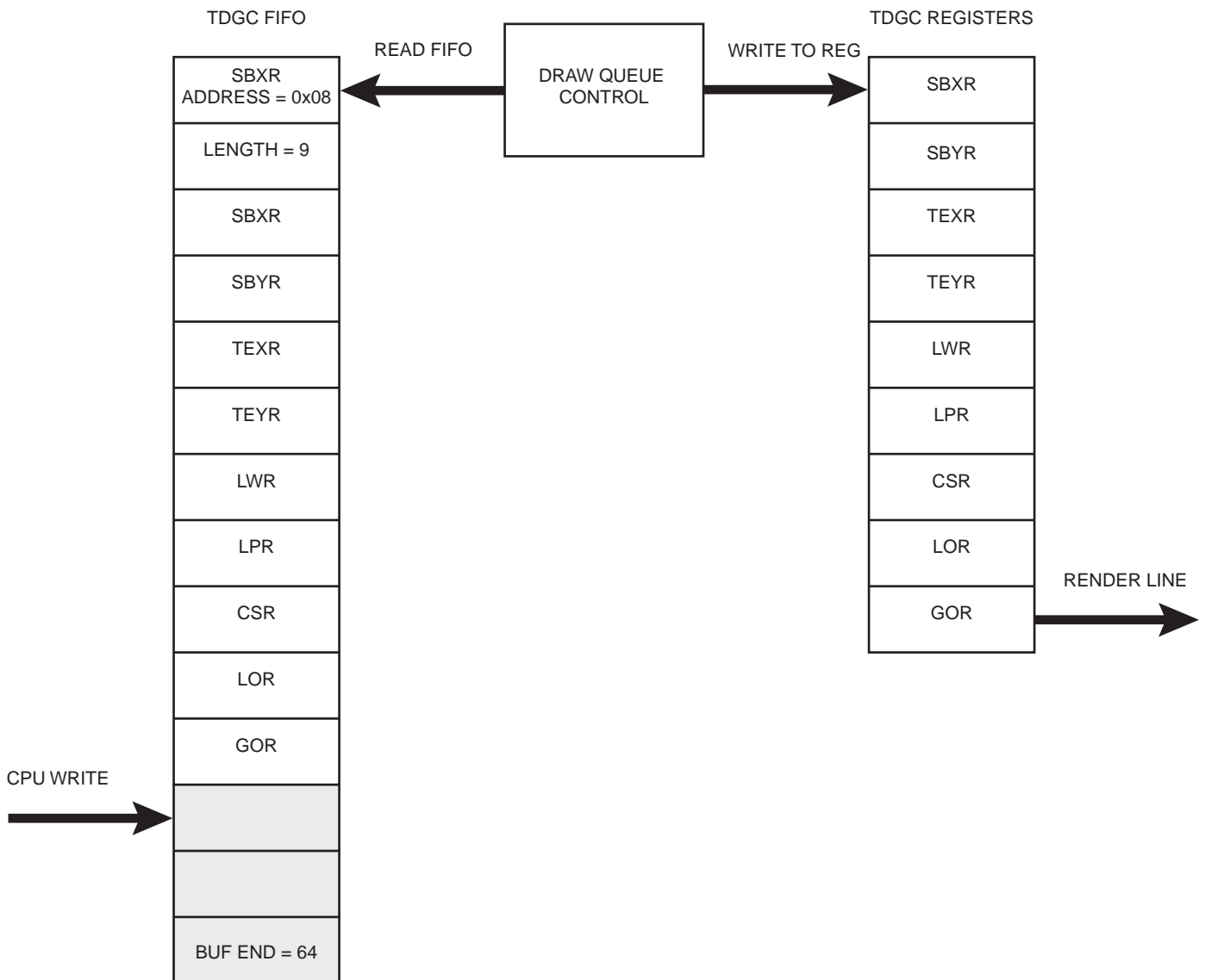
Figure 44-11. Command Queuing
