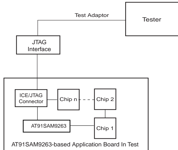
Figure 11-3. Application Test Environment Example
