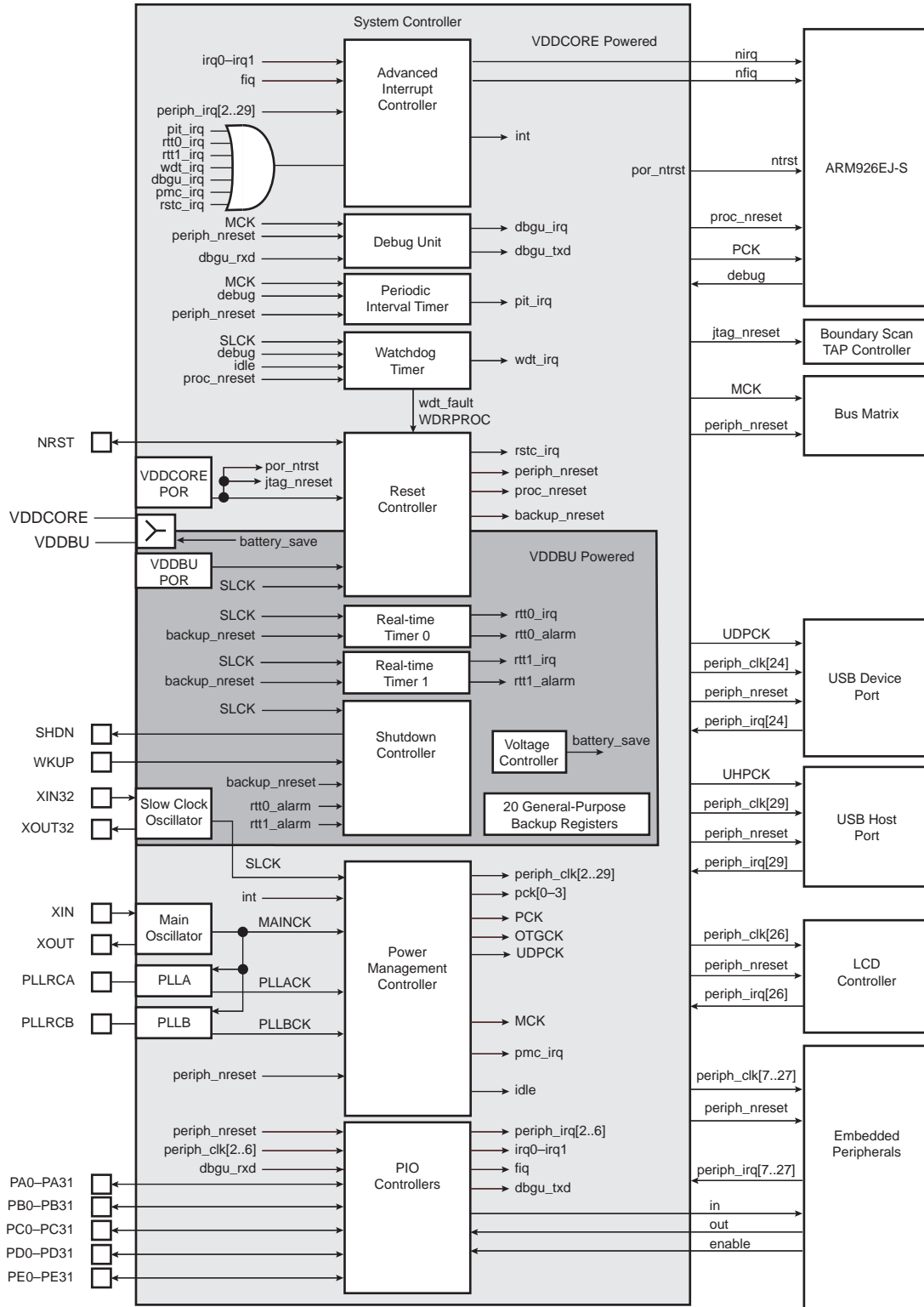
Figure 8-1. SAM9263 System Controller Block Diagram
