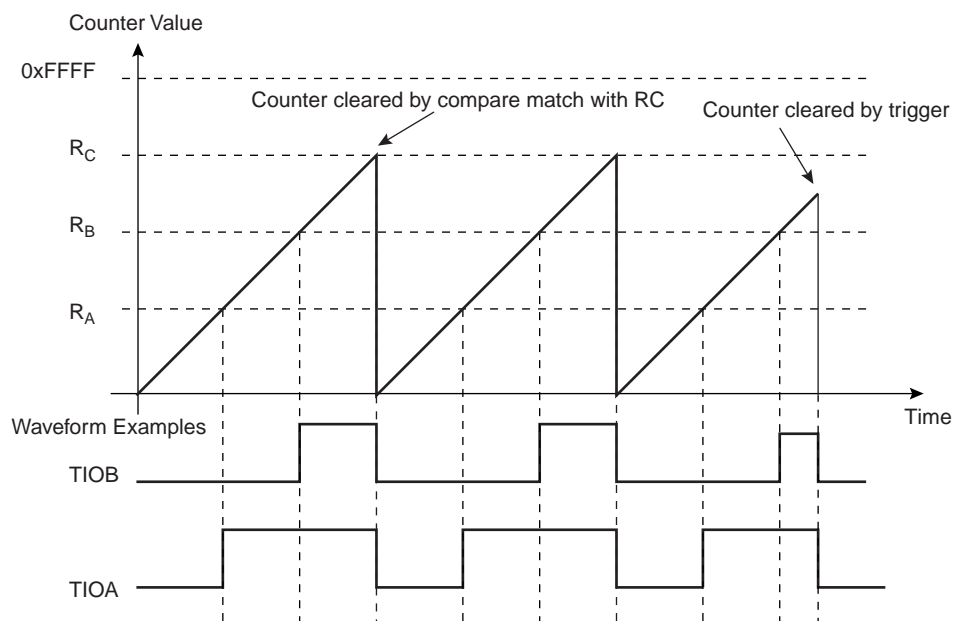
Figure 38-10. WAVSEL = 10 With Trigger
