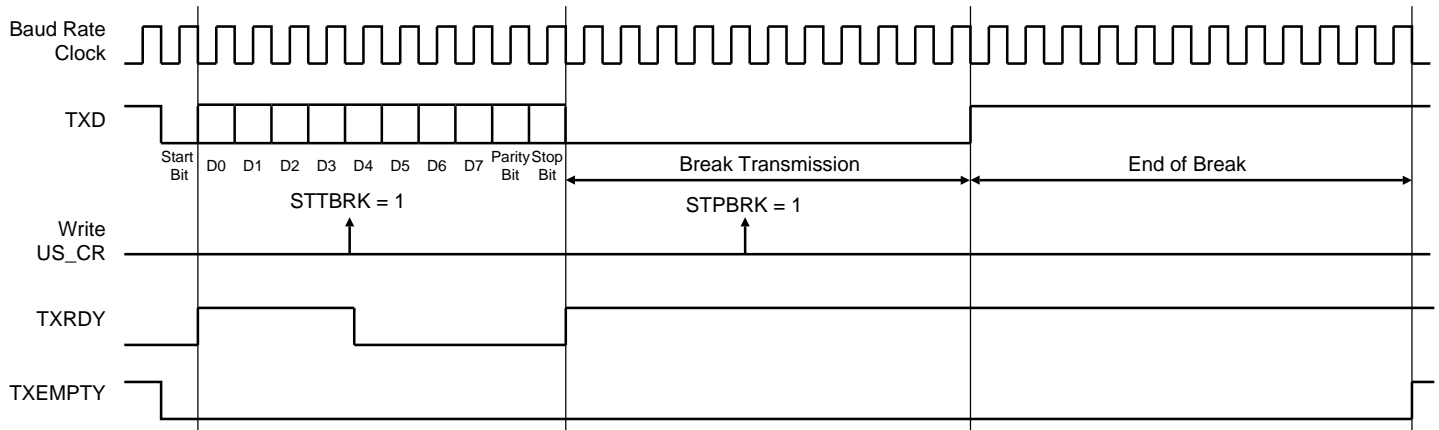
Figure 33-16. Break Transmission
