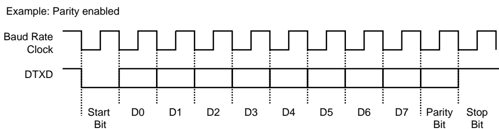
Figure 29-10. Character Transmission
