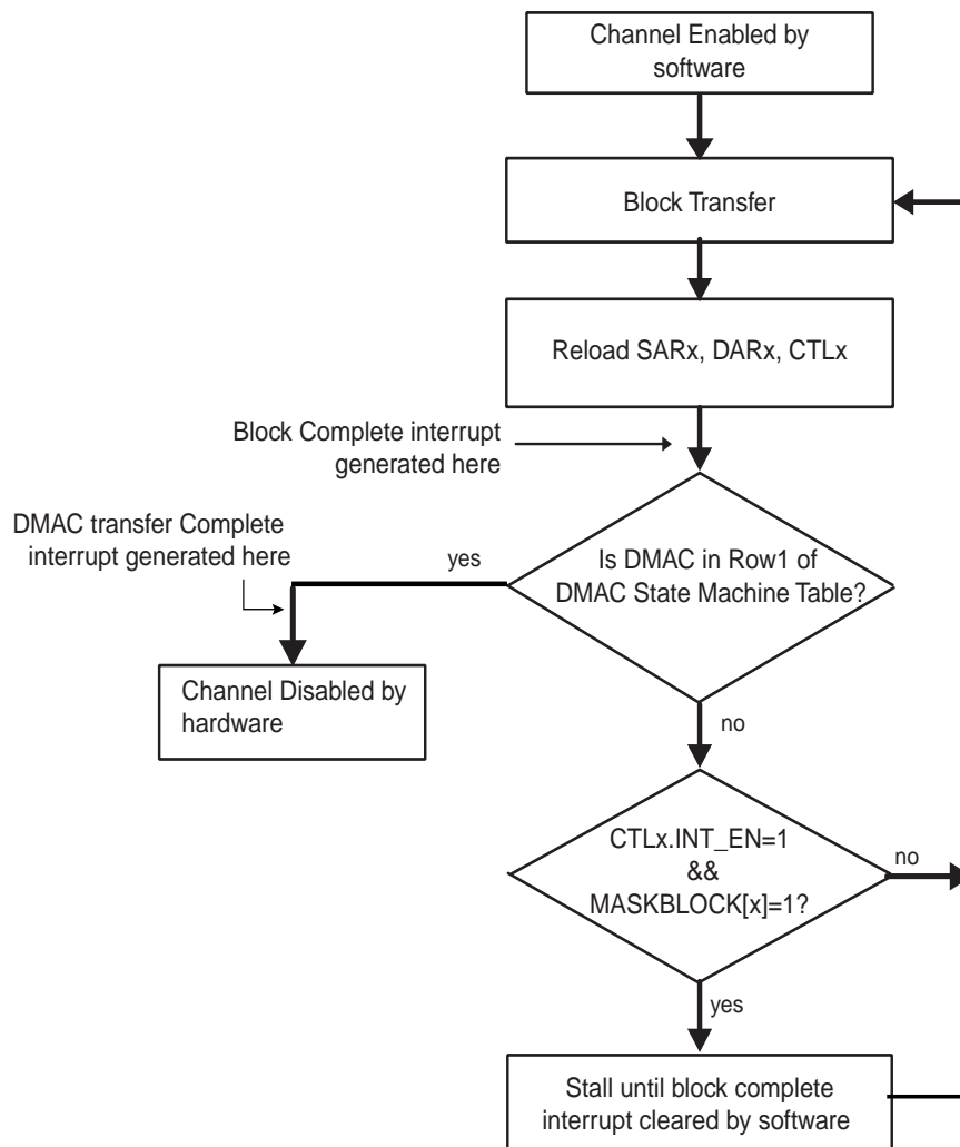
Figure 24-10. DMA Transfer Flow for Source and Destination Address Auto-reloaded
