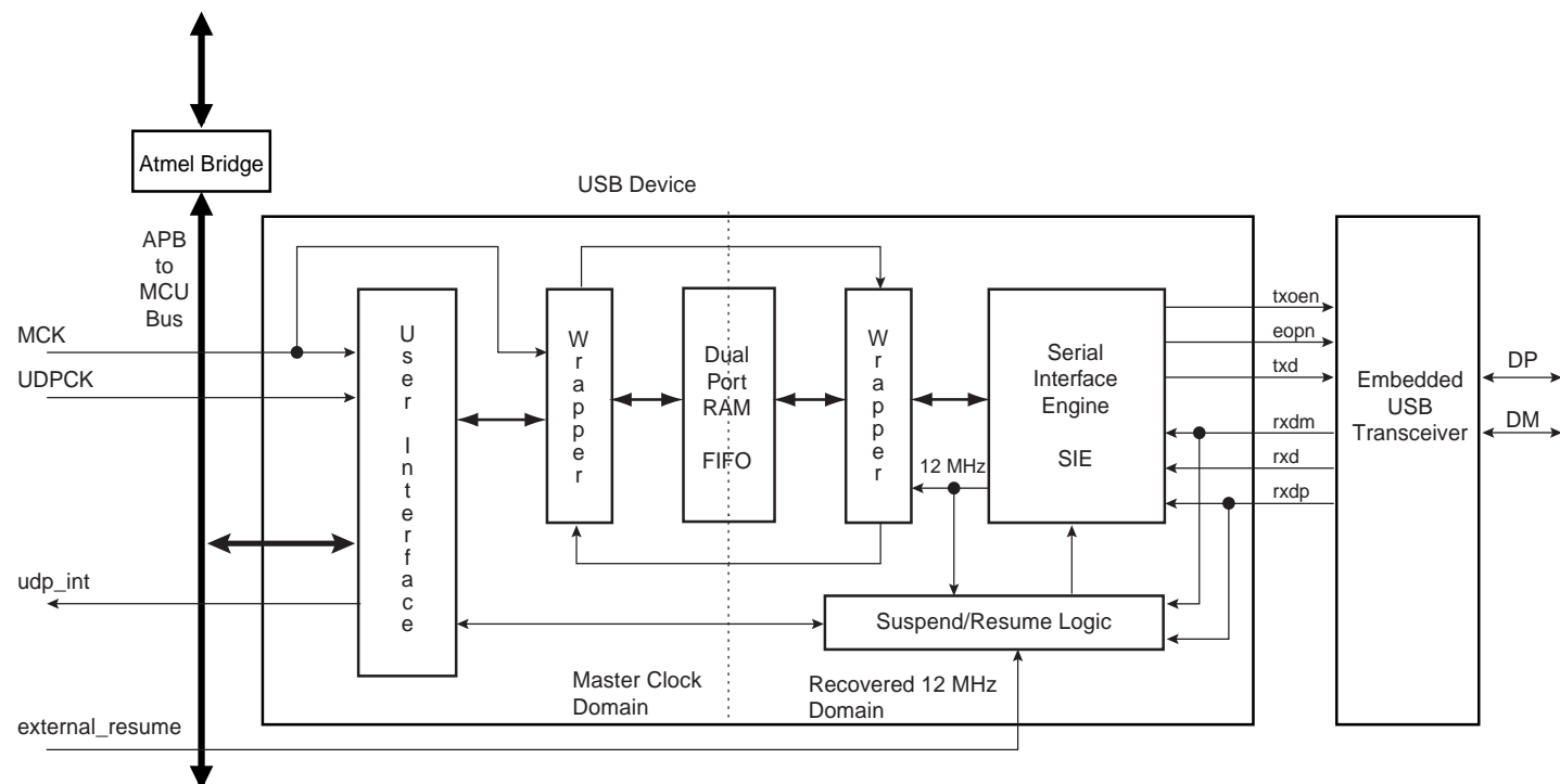
Figure 42-1. Block Diagram
