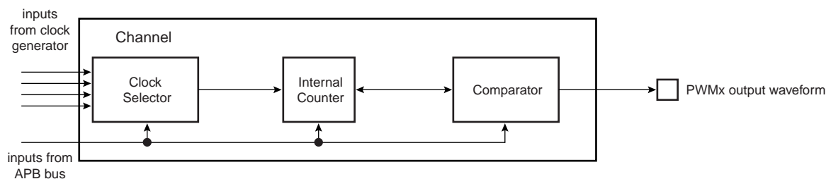
Figure 37-3. Functional View of the Channel Block Diagram
