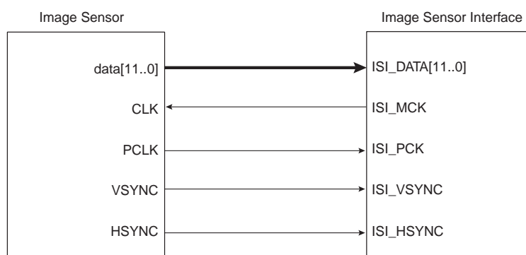
Figure 45-1. ISI Connection Example
