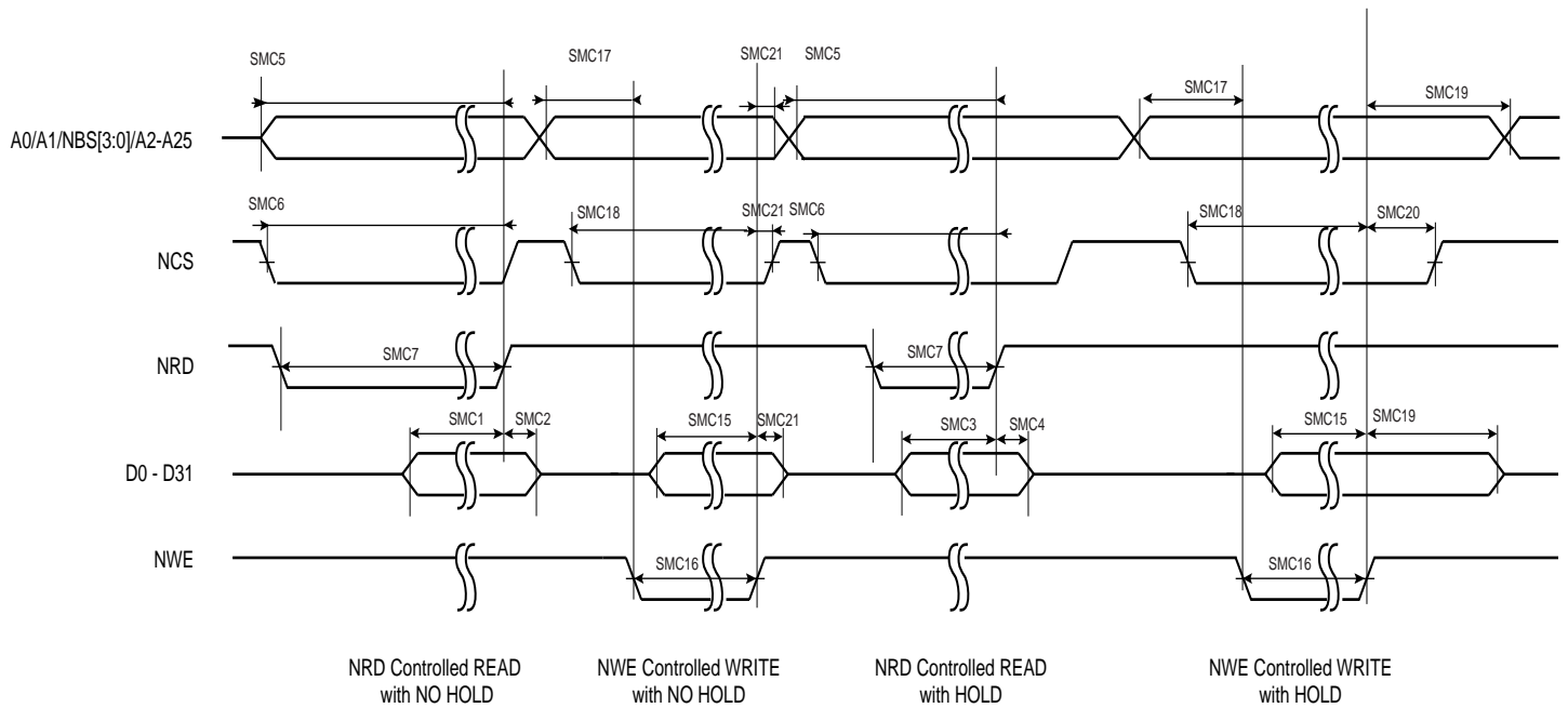
Figure 46-5. SMC timings - NRD controlled Read and NWE controlled Write
