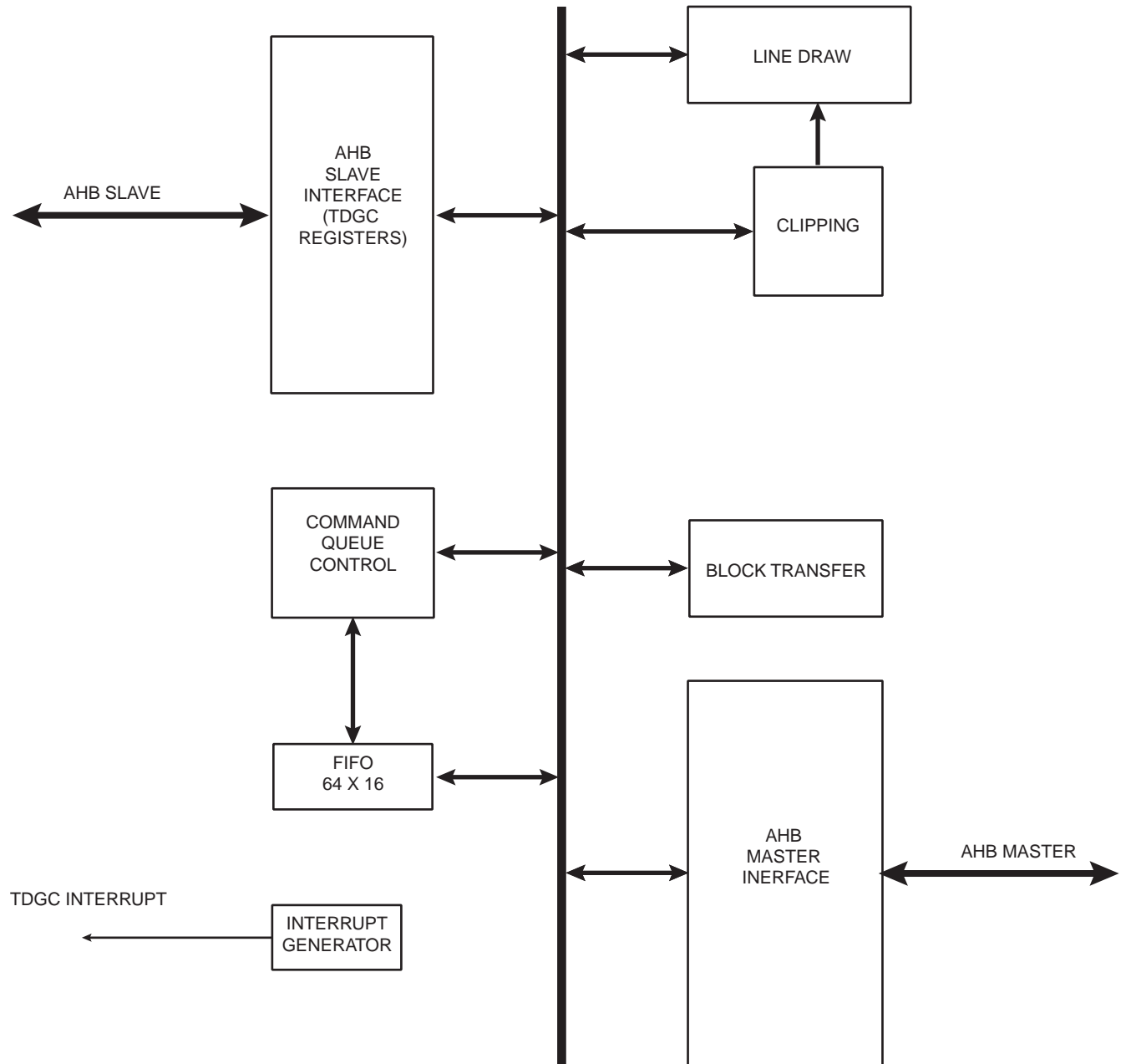
Figure 44-1. Two D Graphic Controller (TGDC) Block Diagram
