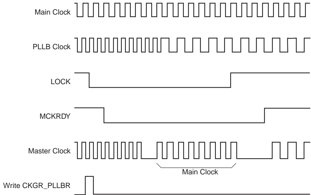
Figure 27-6. Change PLLB Programming
