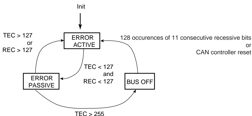
Figure 36-7. Line Error Mode
