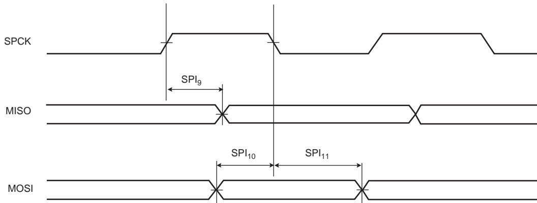
Figure 46-13. SPI Slave Mode 1 and 2
