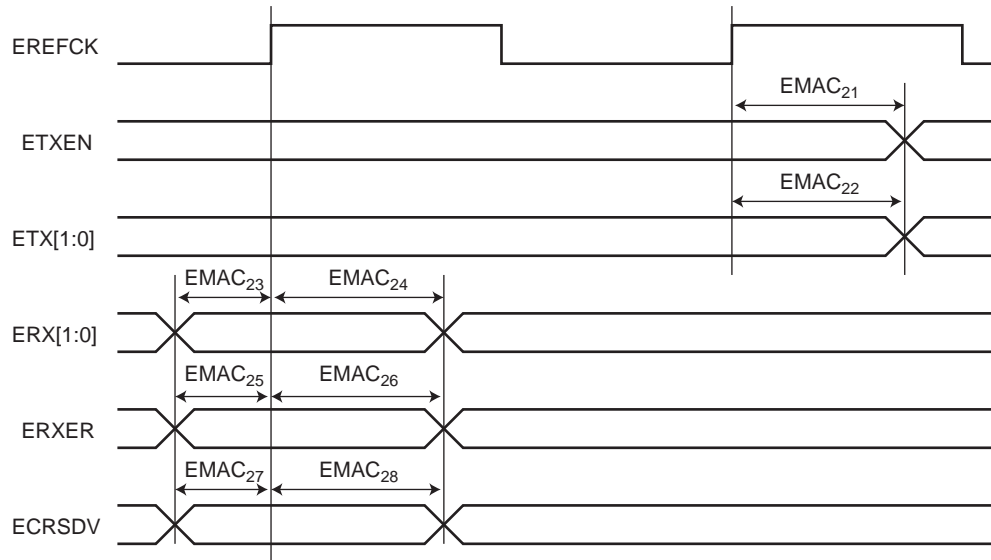
Figure 46-8. EMAC RMII Mode
