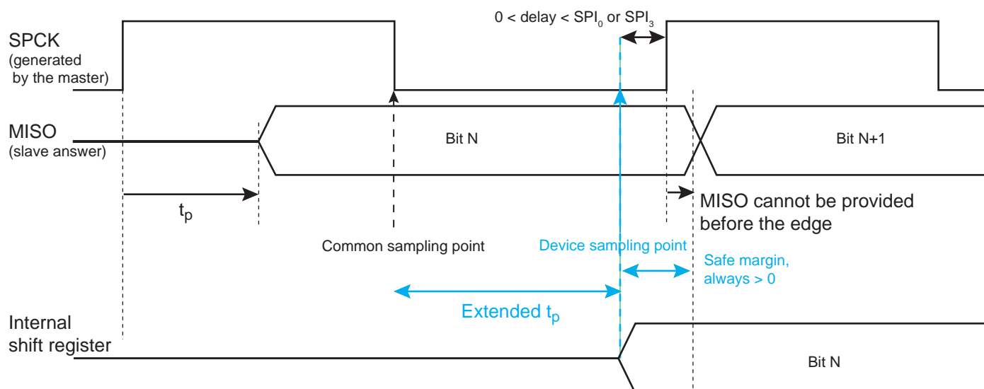
Figure 46-9. MISO Capture in Master Mode
