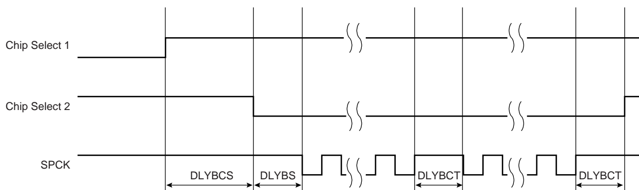
Figure 31-7. Programmable Delays
