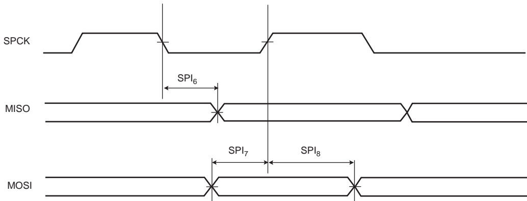
Figure 46-12. SPI Slave Mode 0 and 3
