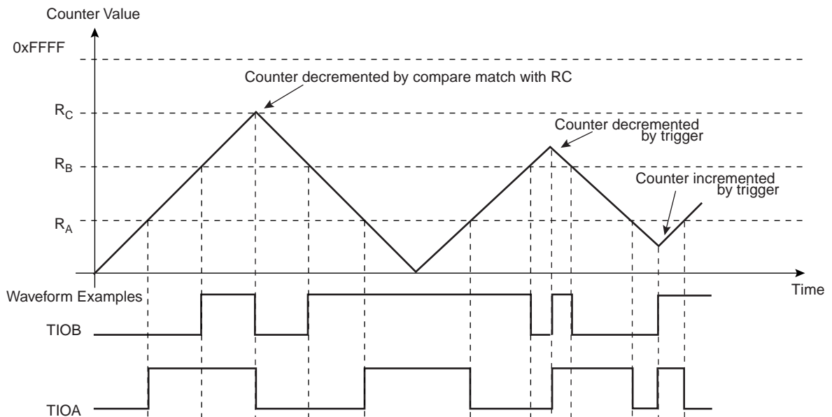
Figure 38-14. WAVSEL = 11 With Trigger
