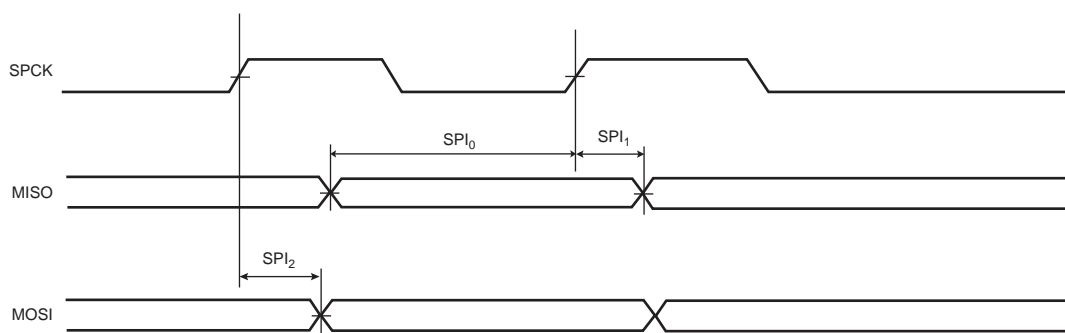
Figure 46-10. SPI Master Mode with (CPOL = 0 and NCPHA = 1) or (CPOL = 1 and NCPHA = 0)
