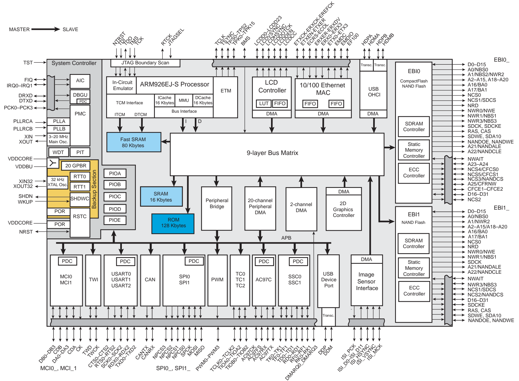
Figure 1-1. SAM9263 Block Diagram
