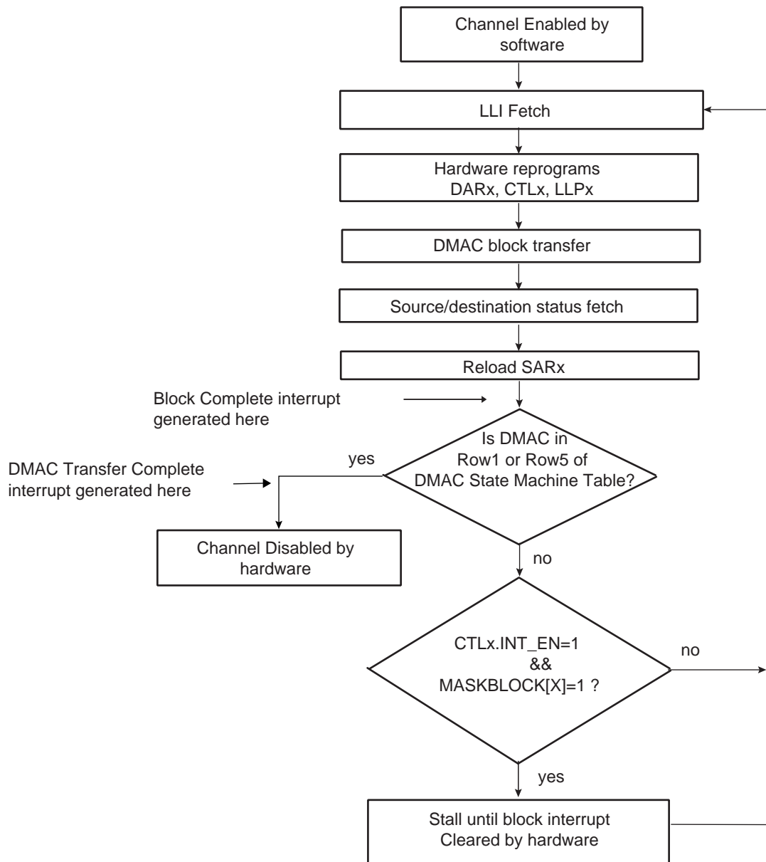
Figure 24-12. DMA Transfer Flow for Source Address Auto-reloaded and Linked List Destination Address
