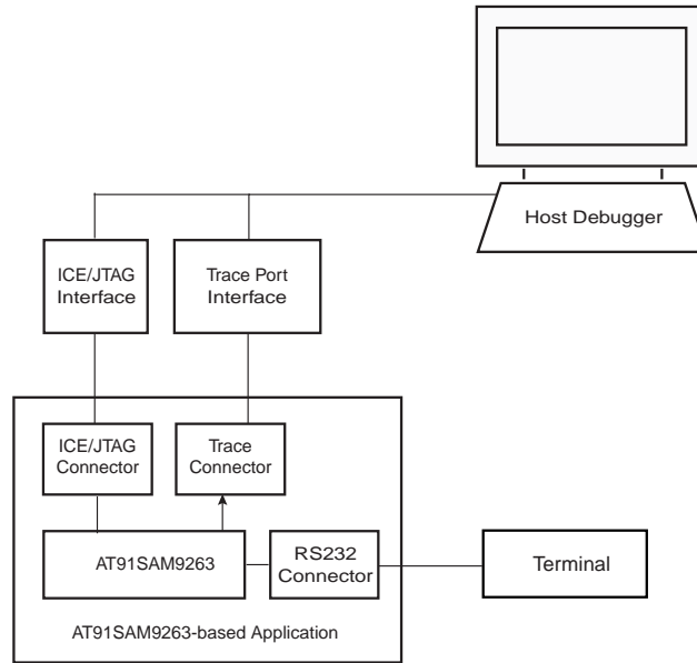
Figure 11-2. Application Debug and Trace Environment Example
