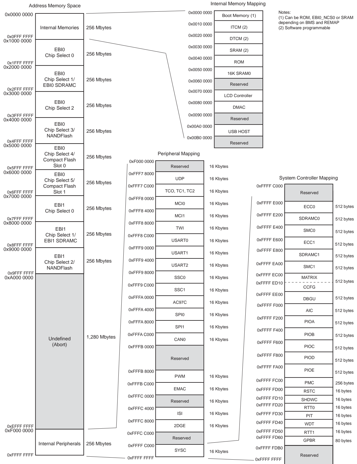
Figure 7-1. SAM9263 Memory Mapping
