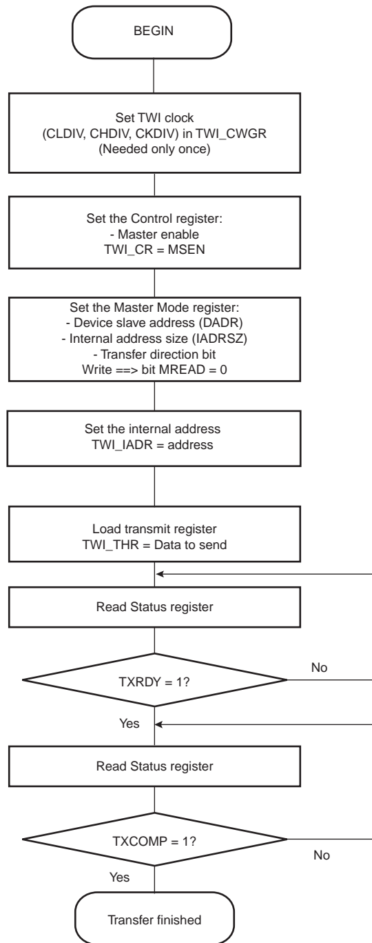
Figure 32-14. TWI Write Operation with Single Data Byte and Internal Address
