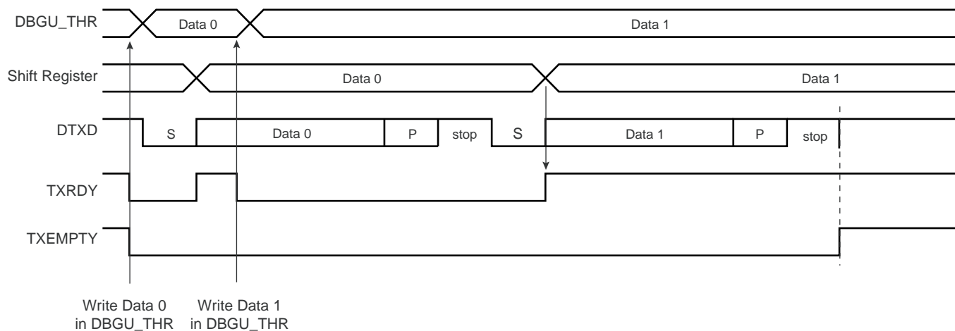
Figure 29-11. Transmitter Control
