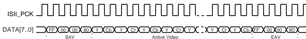
Figure 45-4. SAV and EAV Sequence Synchronization
