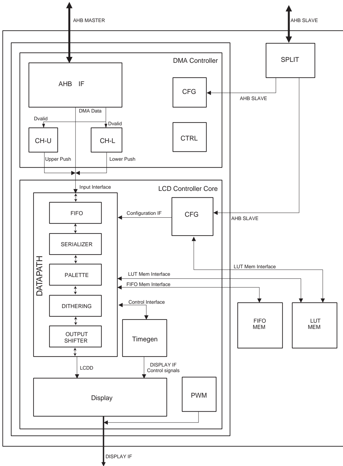
Figure 43-1. LCD Macrocell Block Diagram
