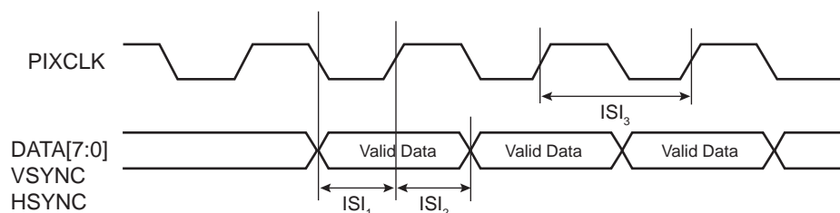
Figure 46-14. ISI Timing Diagram
