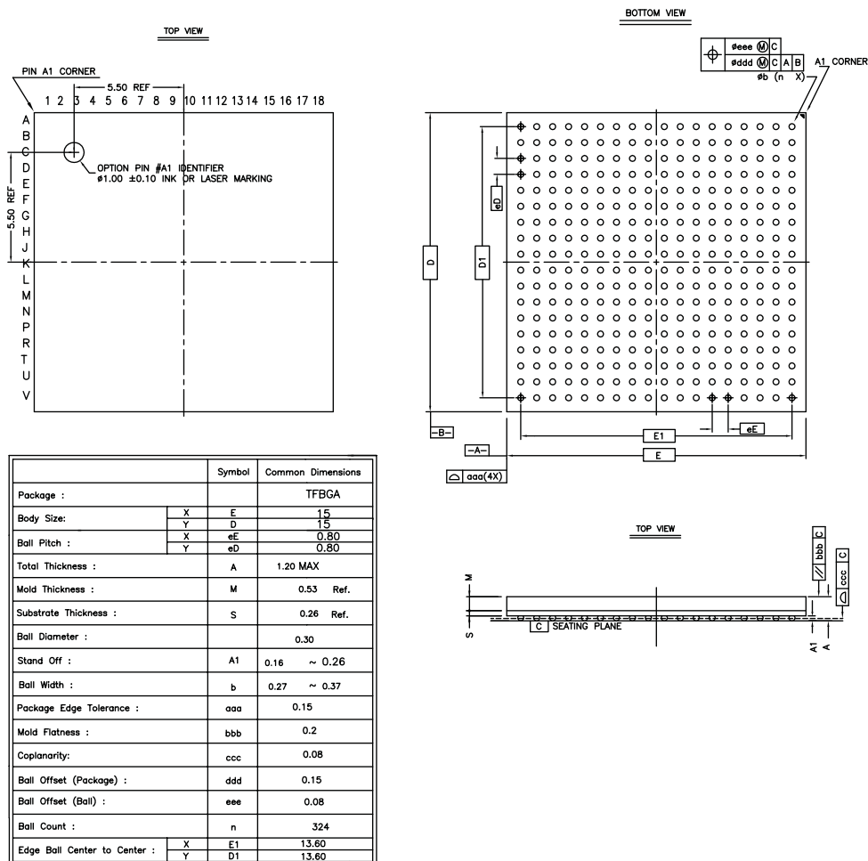
Figure 47-2. 324-ball TFBGA Package Drawing
