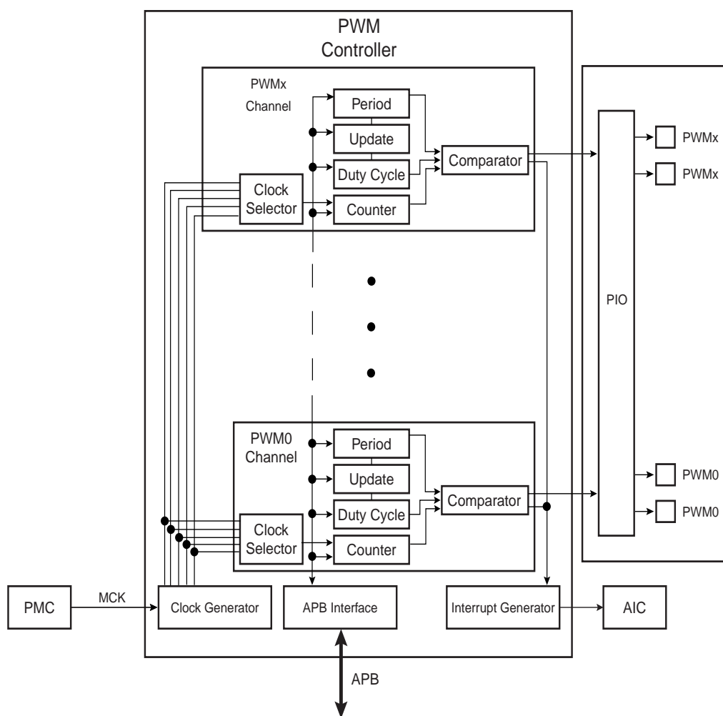
Figure 37-1. Pulse Width Modulation Controller Block Diagram
