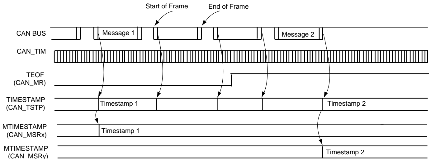
Figure 36-19. Mailbox Timestamp
