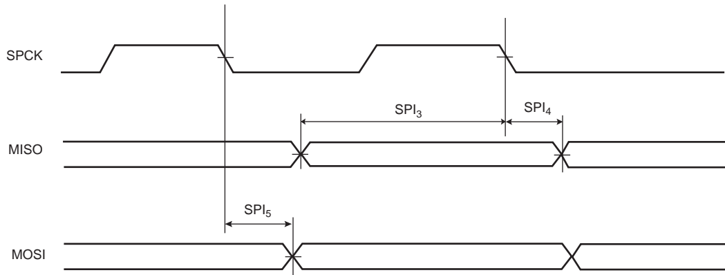
Figure 46-11. SPI Master Mode with (CPOL = NCPHA = 0) or (CPOL = NCPHA = 1)
