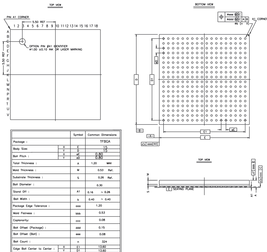
Figure 47-1. 324-ball TFBGA Package Drawing
