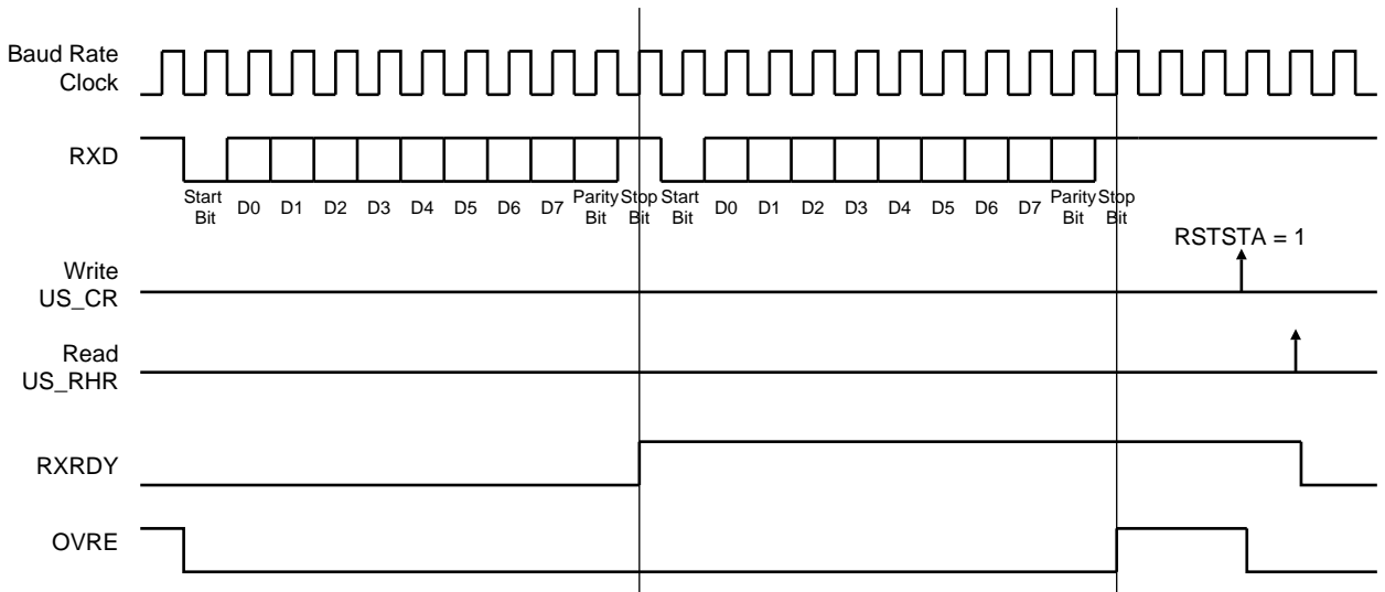
Figure 33-11. Receiver Status
