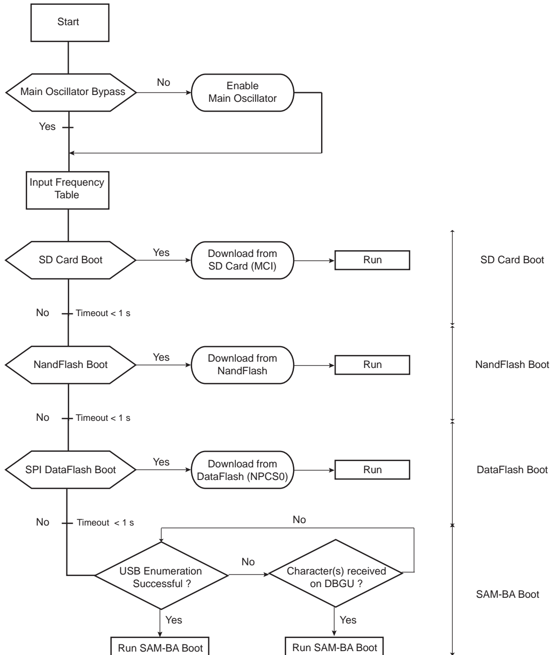
Figure 12-1. Boot Program Algorithm Flow Diagram
