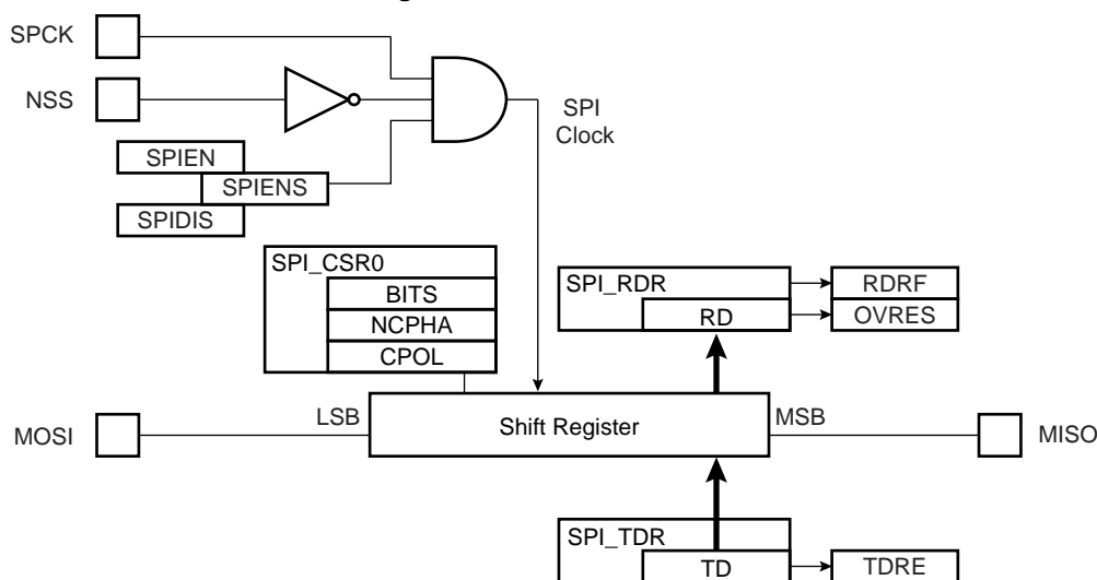
Figure 31-9. Slave Mode Functional Bloc Diagram
