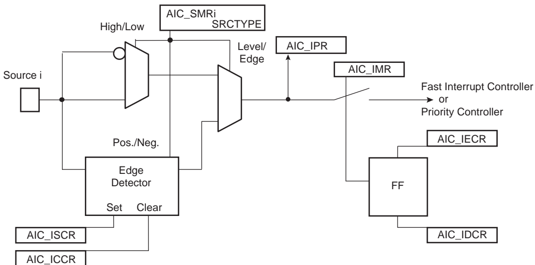
Figure 28-5. External Interrupt Source Input Stage
