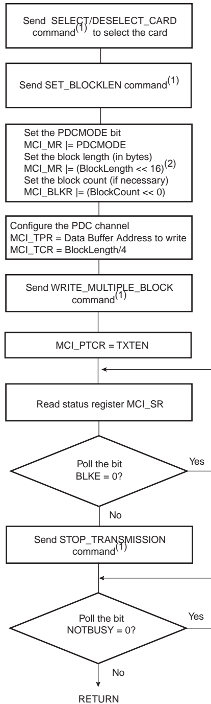
Figure 39-12. Multiple Write Functional Flow Diagram
