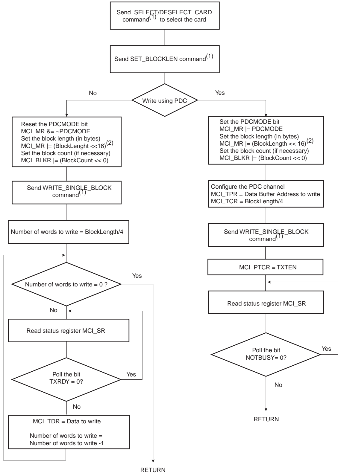
Figure 39-11. Write Functional Flow Diagram
