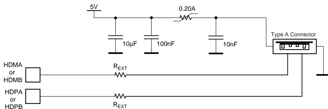
Figure 41-4. Board Schematic to Interface UHP Device Controller
