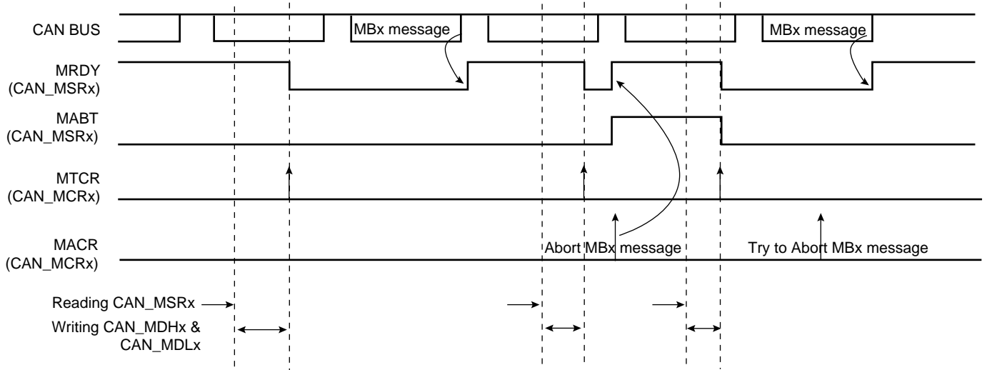
Figure 36-15. Transmitting Messages
