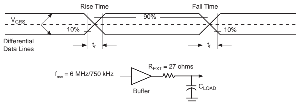
Figure 46-16. USB Data Signal Timing Diagram
