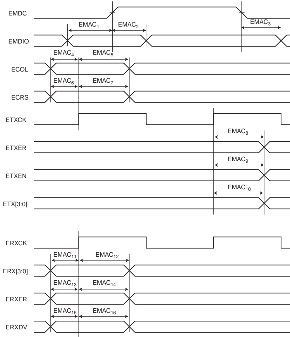
Figure 46-7. EMAC MII Mode
