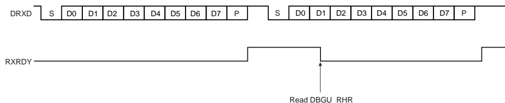
Figure 29-6. Receiver Ready
