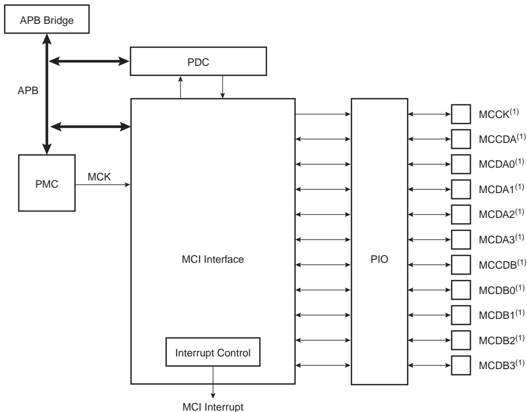
Figure 39-1. Block Diagram
