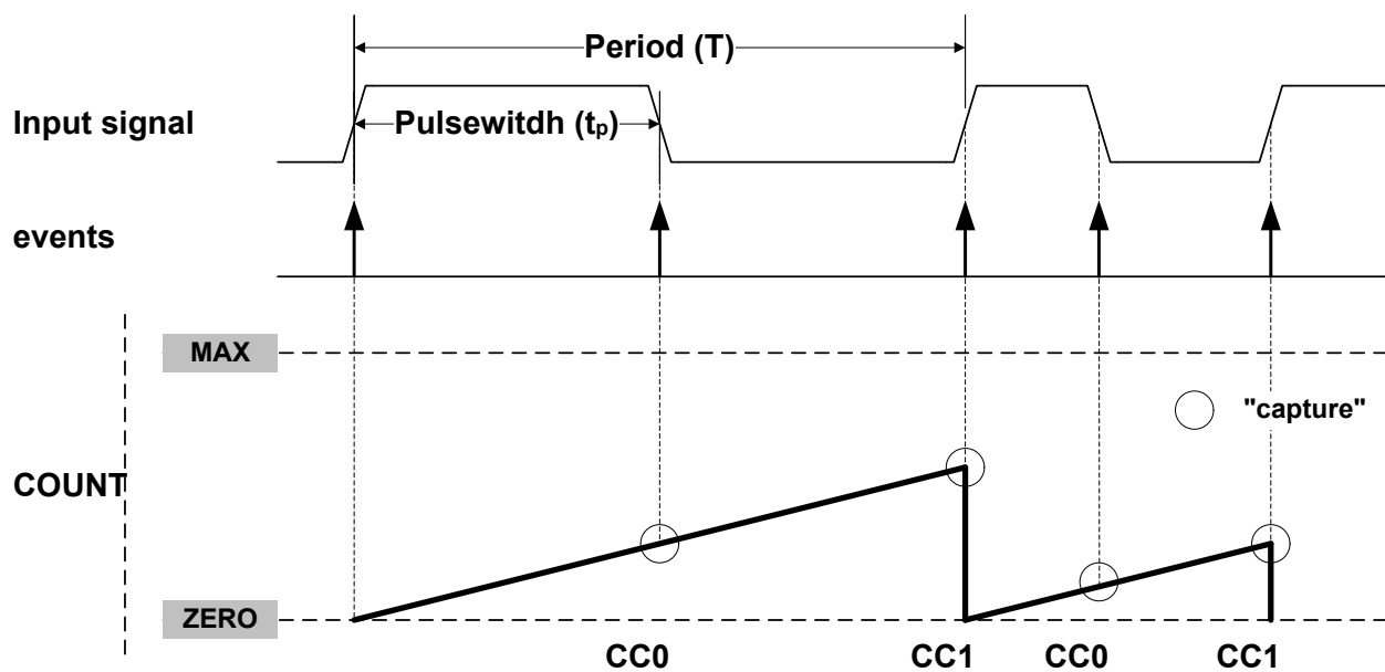
Figure 35-13. PWP Capture
