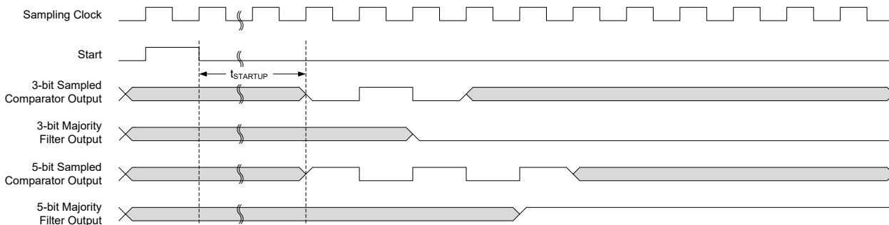
Figure 40-8. Single-Shot Filtering
