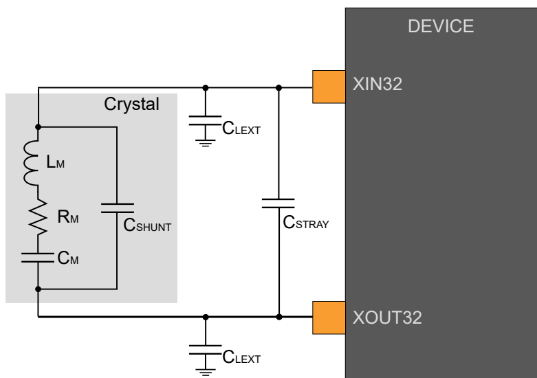
Figure 49-5. Oscillator Connection
