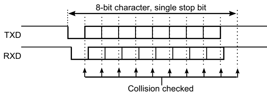
Figure 25-11. Collision Checking
