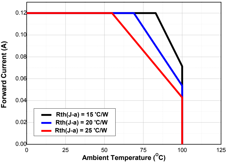
Fig 9. Maximum Forward Current vs. Ambient Temperature, T_j(max.)=125^{\circ}C , I_F=120mA
