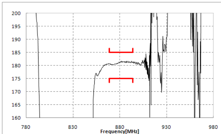
Phase Balance
