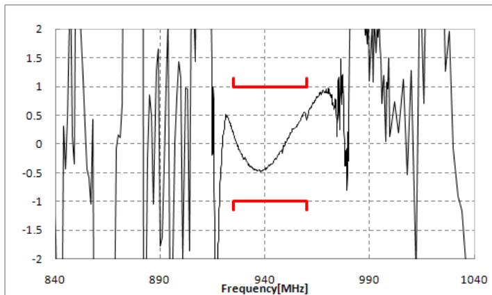
Amplitude Balance
