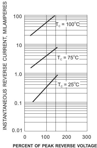
Fig.3- TYPICAL REVERSE CHARACTERISTIC
