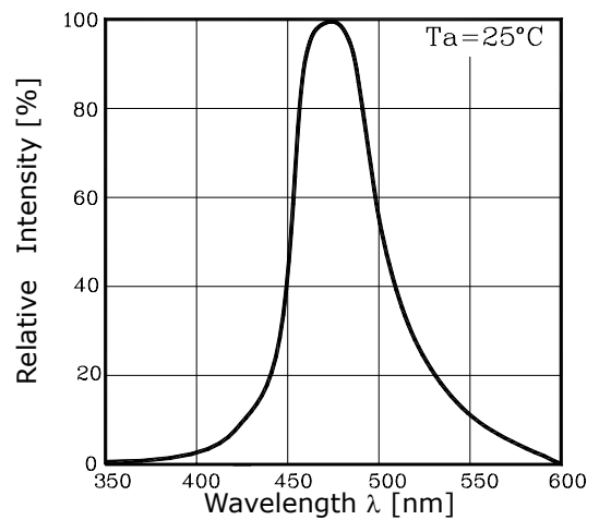
Fig.4 Spectrum Distribution
