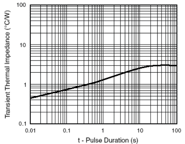
Figure 6. Typical Transient Thermal Impedance Per Diode
