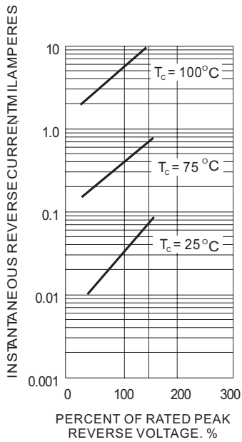
Fig.3-TYPICAL REVERSE CHARACTERISTIC
