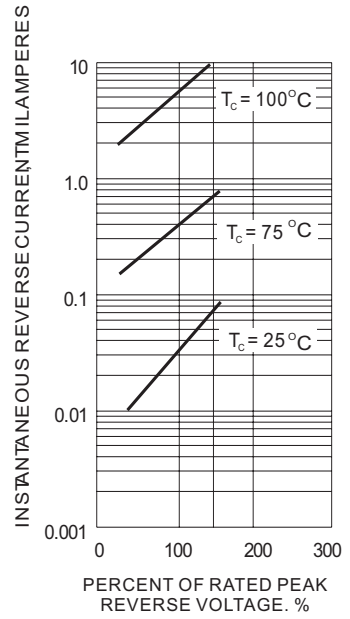
Fig.3-TYPICAL REVERSE CHARACTERISTIC
