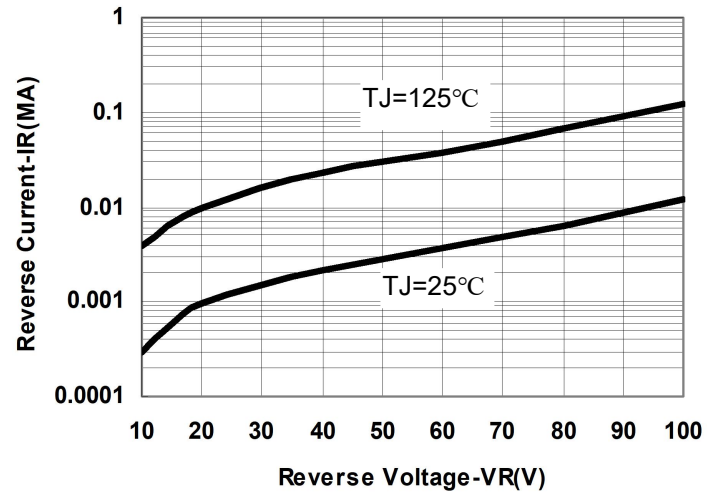
Fig.2-Typical Reverse Current
