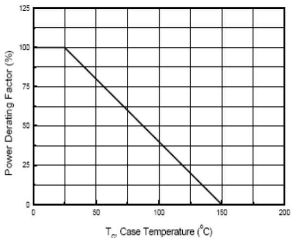
Fig.5 Power Derating
