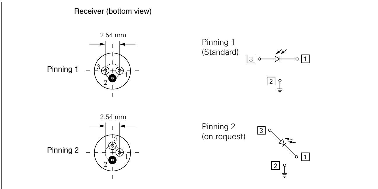
Figure 2 Receiver
