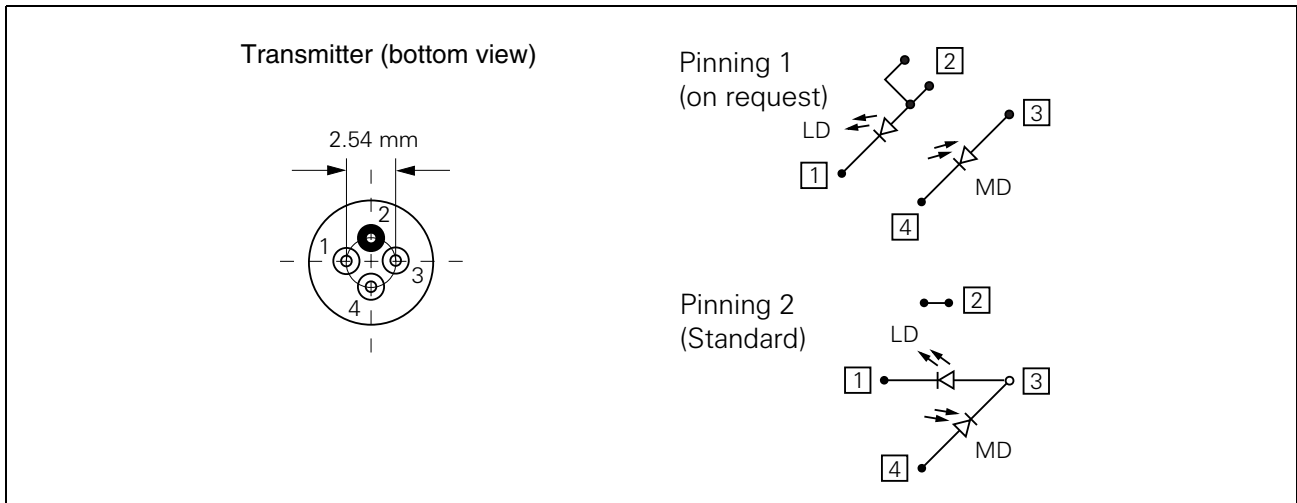
Figure 1 Transmitter
