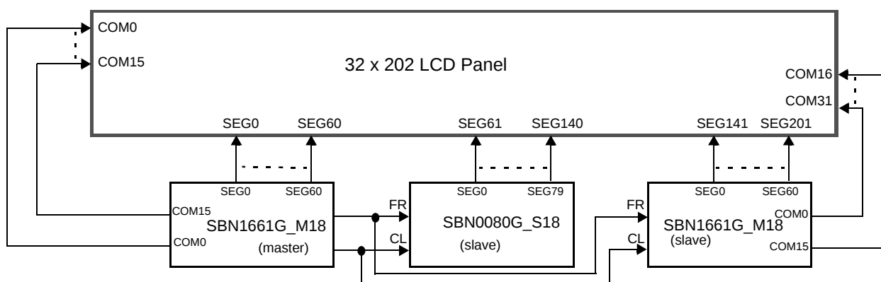
Fig.34 1/32 duty, 33 characters x 4 lines
