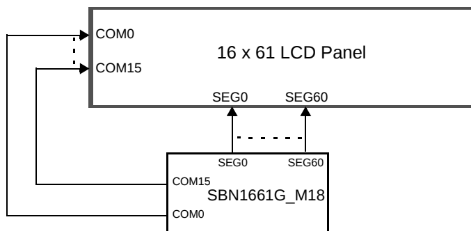
Fig.32 1/16 duty, 10 characters x 2 lines
