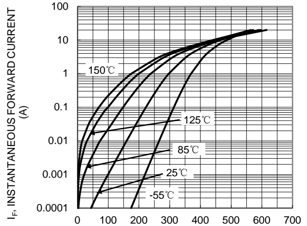
V_F , INSTANTANEOUS FORWARD VOLTAGE (mV) Figure 2. Typical Forward Characteristics
