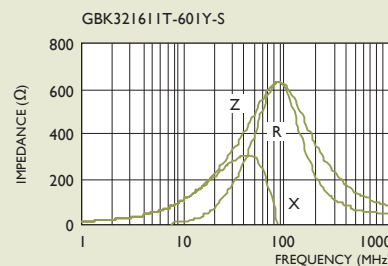
RDC < 0.20Ω Rated Current: 500mA
