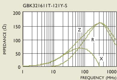
RDC < 0.10 Rated Current: 800mA
