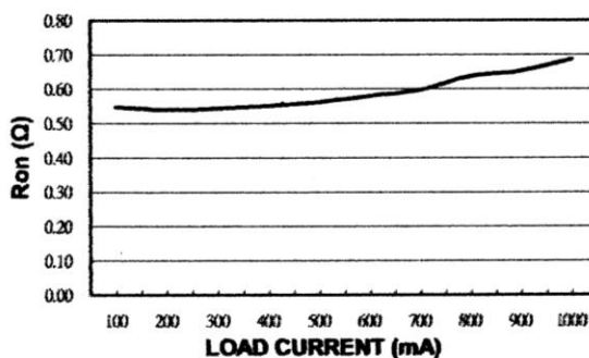
Ron vs. LOAD CURRENT
