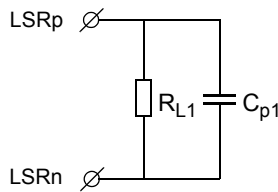
Figure 30: Load circuit A: Dynamic loudspeaker
