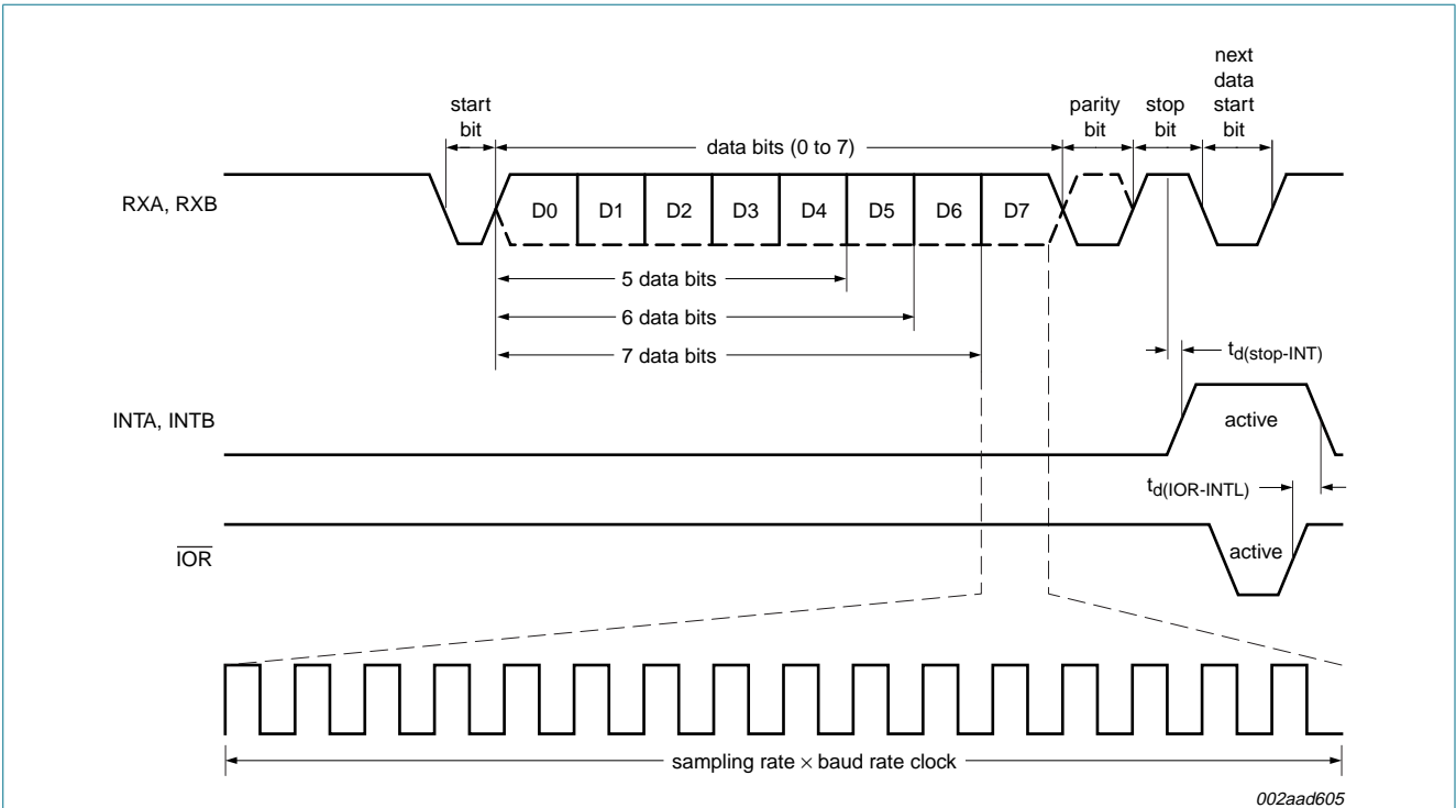
Fig 12. Receive timing
