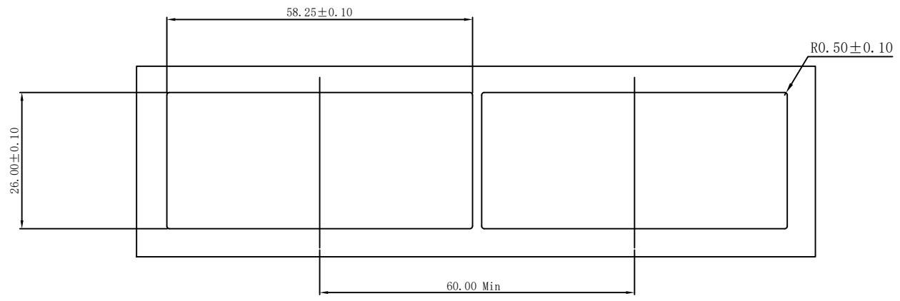
BEZEL CUT-OUT CENTER SPACING DETAIL BEZEL THICKNESS: 0.8-2.6
