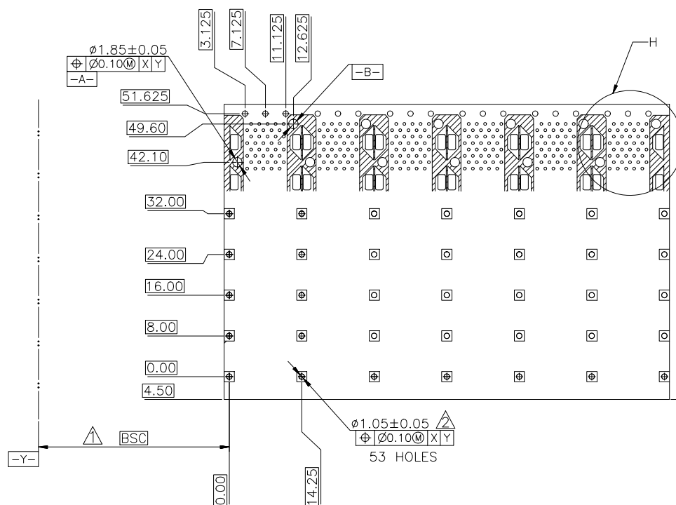
ECOMMENDED PCB CONFIGURATION
