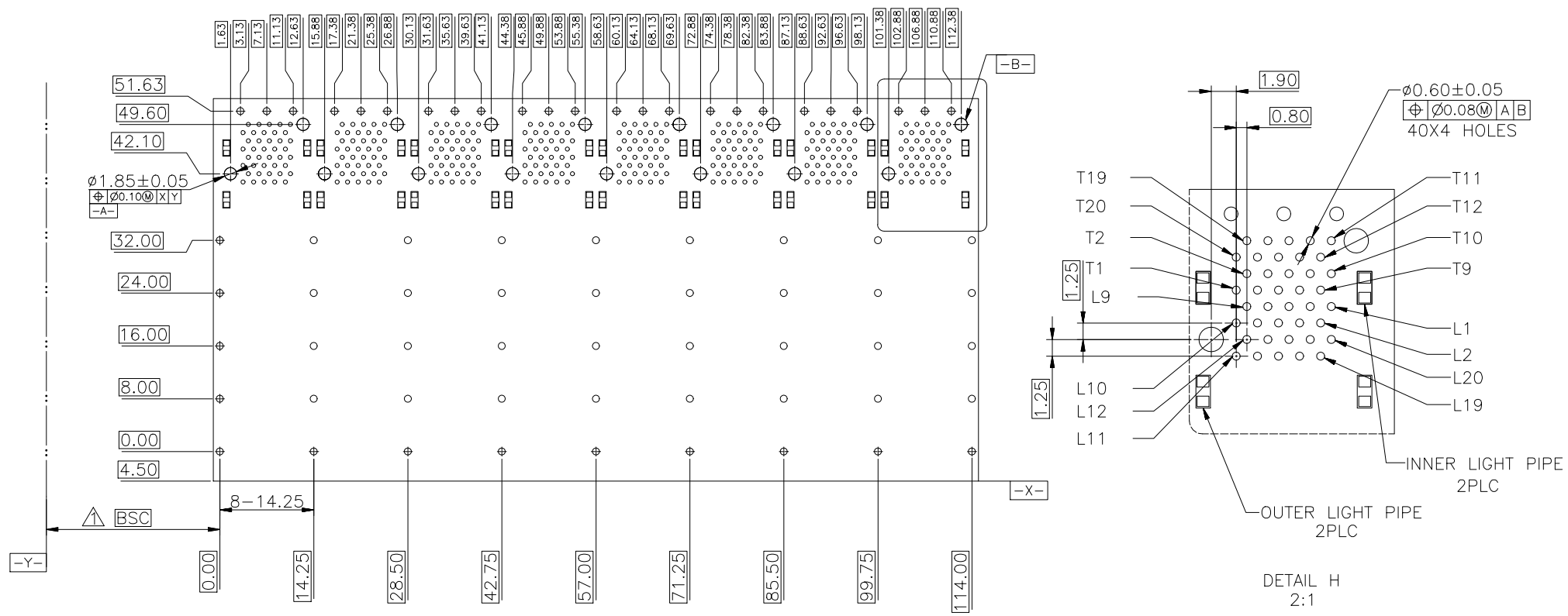
ECOMMENDED PCB CONFIGURATION
