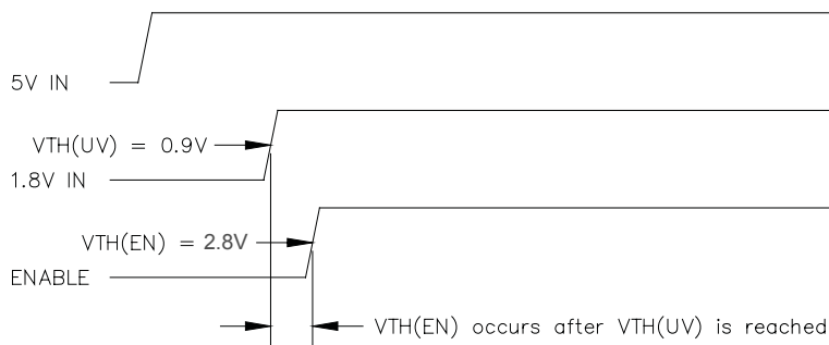
SC339 Supply Comes Up Before MOSFET Drain Supply
