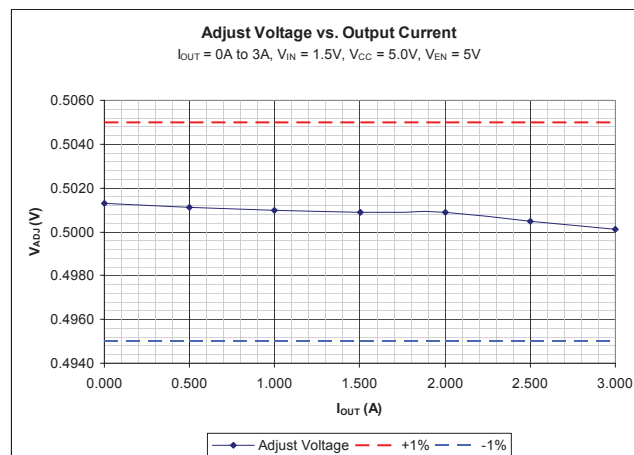
Figure 2: Adjust Voltage v/s Output Current (1% accurate)
