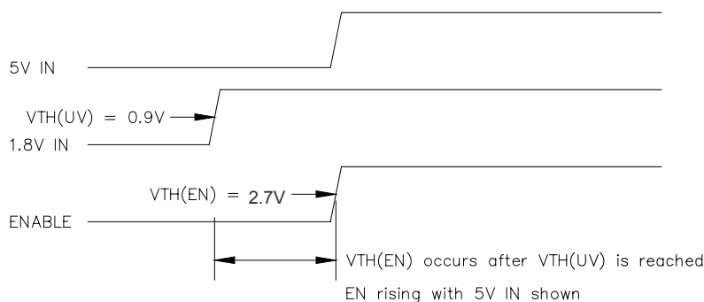
MOSFET Drain Supply Comes Up Before SC339 Supply
