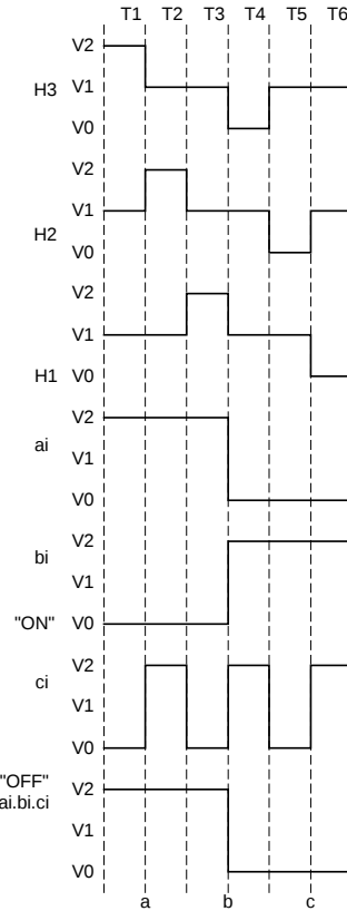
No. "5" ON OR OFF WAVEFORM
