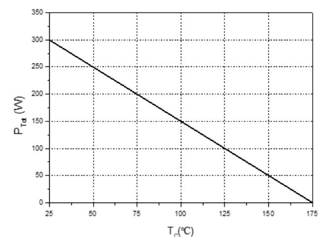
Power Derating
