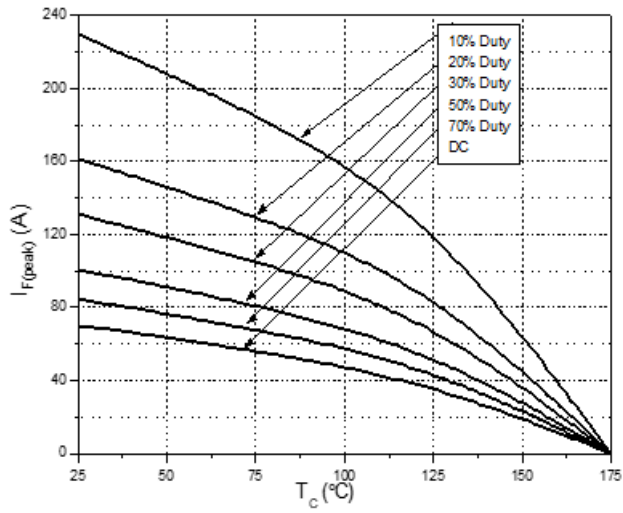
Current Derating
