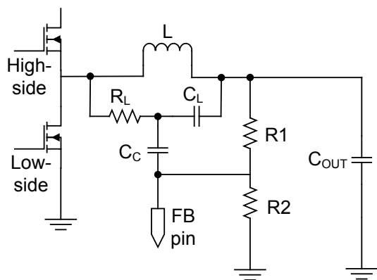
Figure 11 — Signal Injection Circuit
