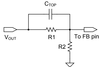
Figure 10 — Capacitor Coupling to FB Pin
