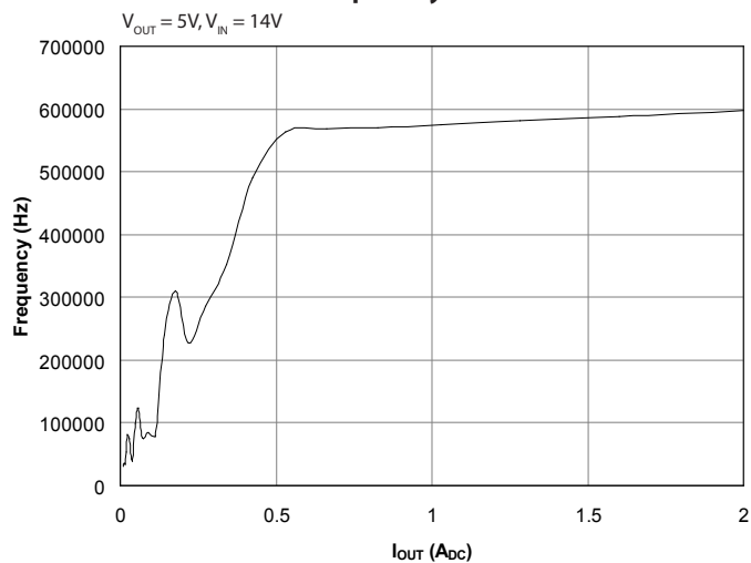
Frequency vs. Load
