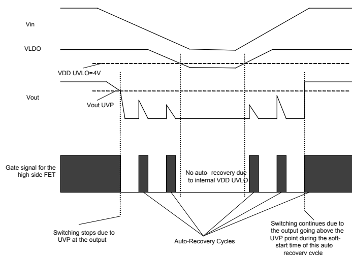
Figure 8 — Auto Recovery Due to Input UVLO
