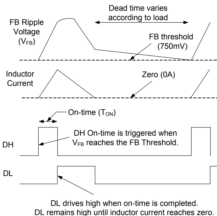
Figure 5 — Power Save Operation
