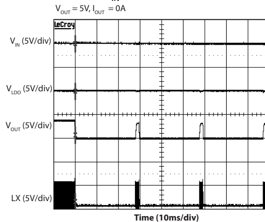
V_{IN} Variation - Zoom
