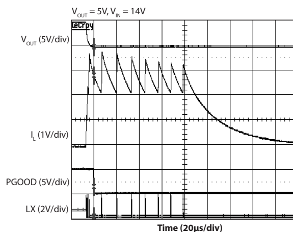
Over Current - Short Circuit
