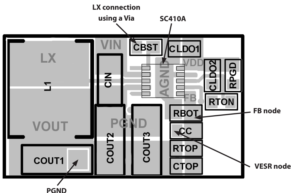
Figure 12 — PCB Layout
