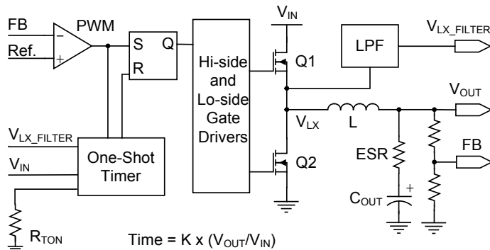
Figure 2 — On-Time Generation
