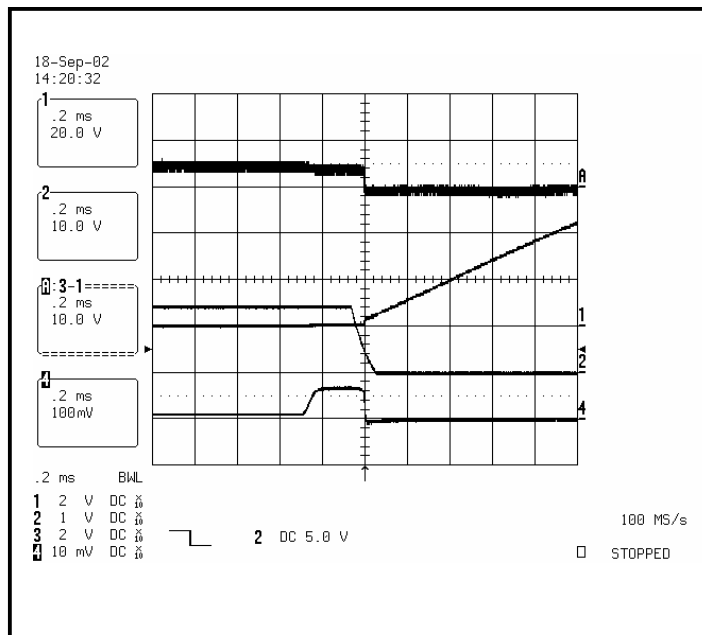
Figure 10. Over-current/Short circuit.
