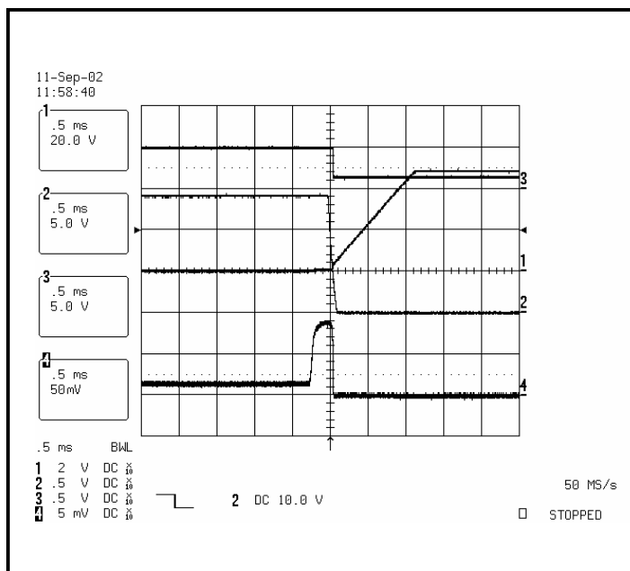
Figure 6. Over-current/Short circuit.
