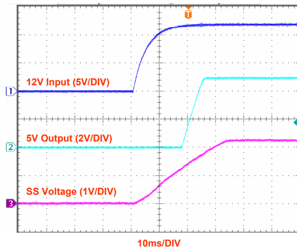
V_{IN} Start up Transient ( I_O=3A )
