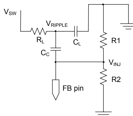
Figure 6 – AC Equivalent Circuit
