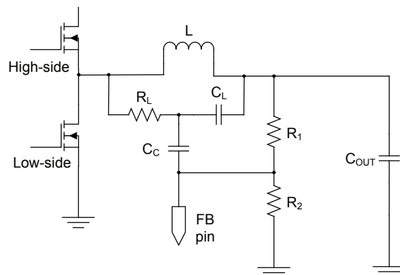
Figure 5 – Virtual ESR Network
