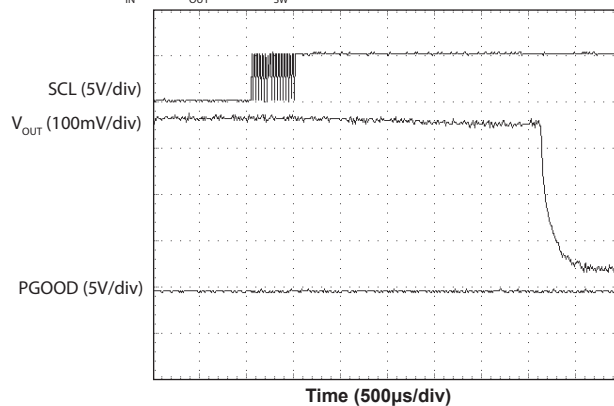
Slew-Down — CCM, No Load, EnIntLd=1
