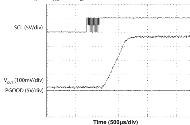
Slew-Up — CCM, No Load, EnIntLd=0/1
