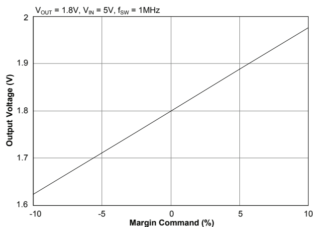
Output Voltage vs. Margin — CCM
