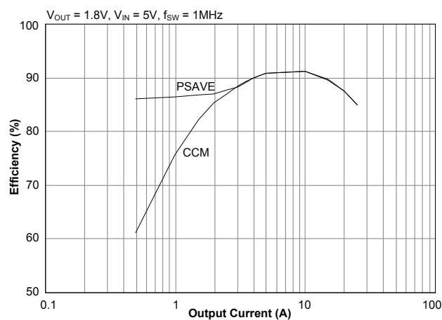
Efficiency vs Load — CCM and PSAVE
