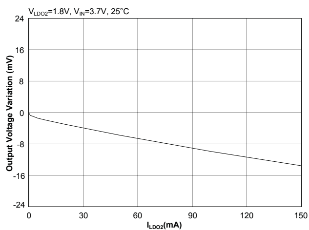
Load Regulation (LDO2)
