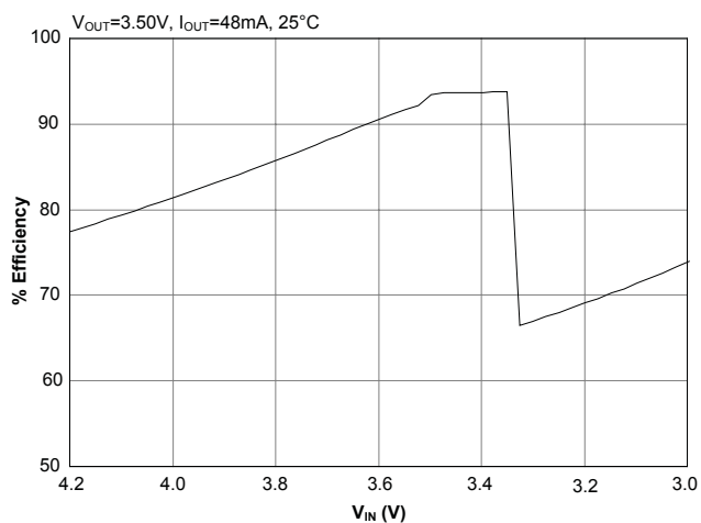
Backlight Efficiency (4 LEDs) — 12mA Each
