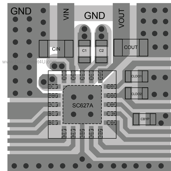
Figure 1 — Recommended PCB Layout
