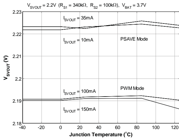
DC/DC Converter Temperature Regulation
