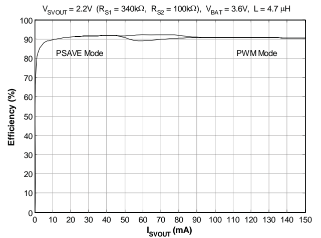
DC/DC Converter Efficiency
