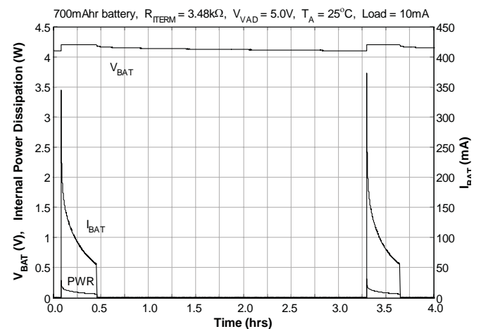
Re-Charge Cycle Battery Voltage and Current
